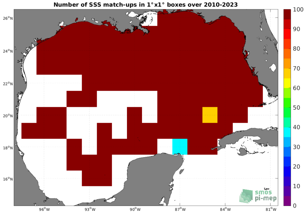
Figure 4: Number of SSS match-ups between TSG (SAMOS) SSS and the SMOS SSS L3 v335 - Monthly - 25 km (CATDS-CPDC) SSS product for the Gulf of Mexico Pi-MEP region over 1^\circ \times 1^\circ boxes and for the full satellite product period.
