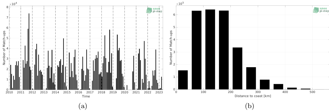
Figure 1: Number of match-ups between TSG (SAMOS) and SMOS SSS L3 v335 - Monthly - 25 km (CATDS-CPDC) SSS as a function of time (a) and as function of the distance to coast (b) over the Gulf of Mexico Pi-MEP region and for the full satellite product period.
