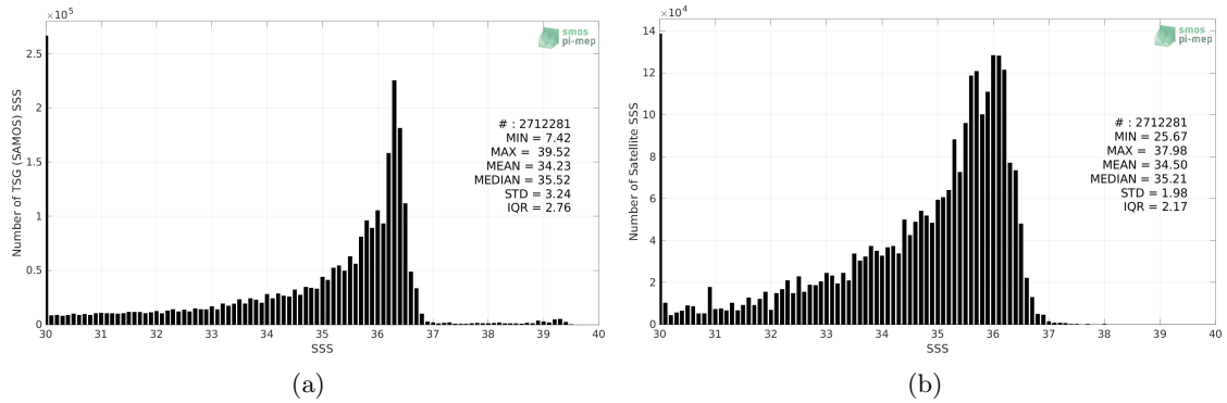
Figure 2: Histograms of SSS from TSG (SAMOS) (a) and SMOS SSS L3 v335 - Monthly - 25 km (CATDS-CPDC) (b) considering all match-up pairs per bins of 0.1 over the Gulf of Mexico Pi-MEP region and for the full satellite product period.
