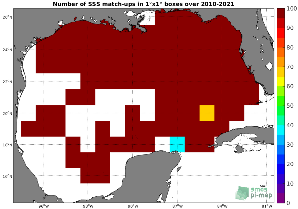
Figure 4: Number of SSS match-ups between TSG (SAMOS) SSS and the SMOS SSS L3 v335 - Monthly - 25 km (CATDS-CPDC) SSS product for the Gulf of Mexico Pi-MEP region over 1^{\circ} \times 1^{\circ} boxes and for the full satellite product period.
