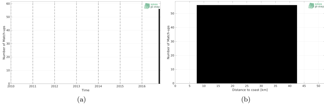
Figure 1: Number of match-ups between TSG (LEGOS-DM) and SMOS SSS L3 v335 - Monthly - 25 km (CATDS-CPDC) SSS as a function of time (a) and as function of the distance to coast (b) over the Gulf of Mexico Pi-MEP region and for the full satellite product period.
