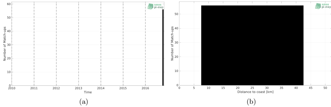
Figure 1: Number of match-ups between TSG (LEGOS-DM) and SMOS SSS L3 v335 - Monthly - 25 km (CATDS-CPDC) SSS as a function of time (a) and as function of the distance to coast (b) over the Gulf of Mexico Pi-MEP region and for the full satellite product period.
