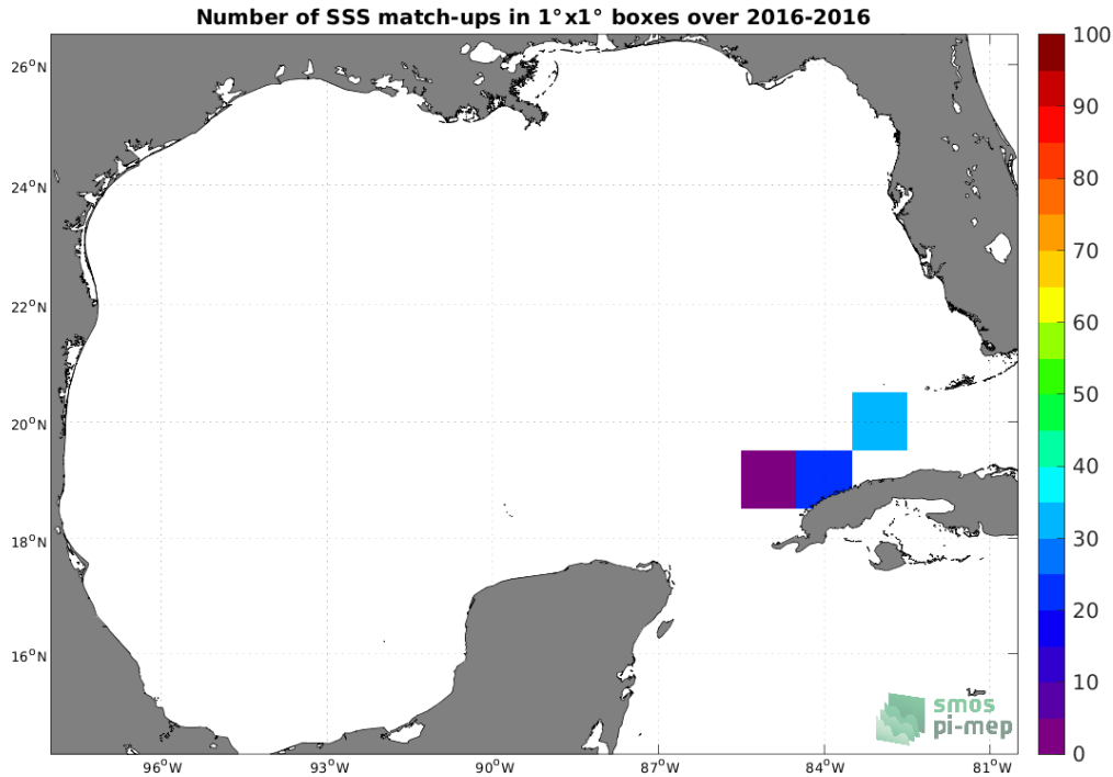
Figure 4: Number of SSS match-ups between TSG (LEGOS-DM) SSS and the SMOS SSS L3 v335 - Monthly - 25 km (CATDS-CPDC) SSS product for the Gulf of Mexico Pi-MEP region over 1^\circ \times 1^\circ boxes and for the full satellite product period.
