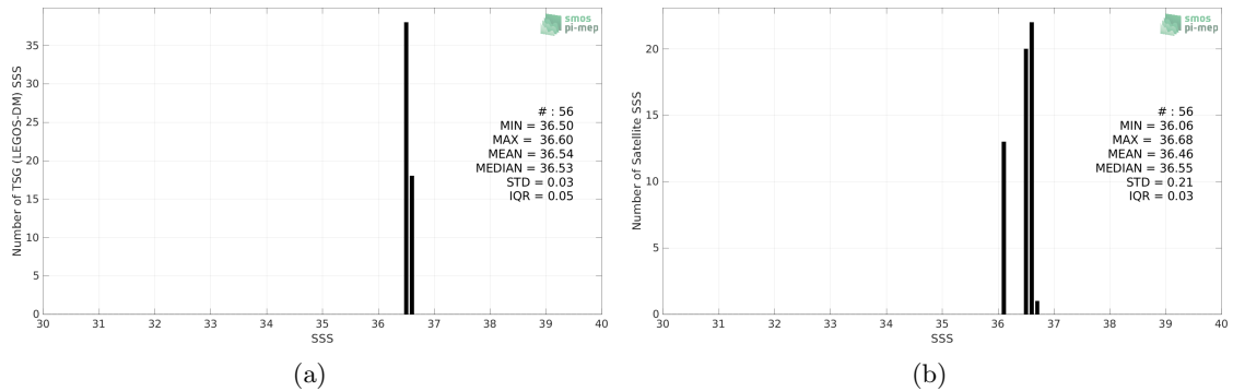
Figure 2: Histograms of SSS from TSG (LEGOS-DM) (a) and SMOS SSS L3 v335 - Monthly - 25 km (CATDS-CPDC) (b) considering all match-up pairs per bins of 0.1 over the Gulf of Mexico Pi-MEP region and for the full satellite product period.
