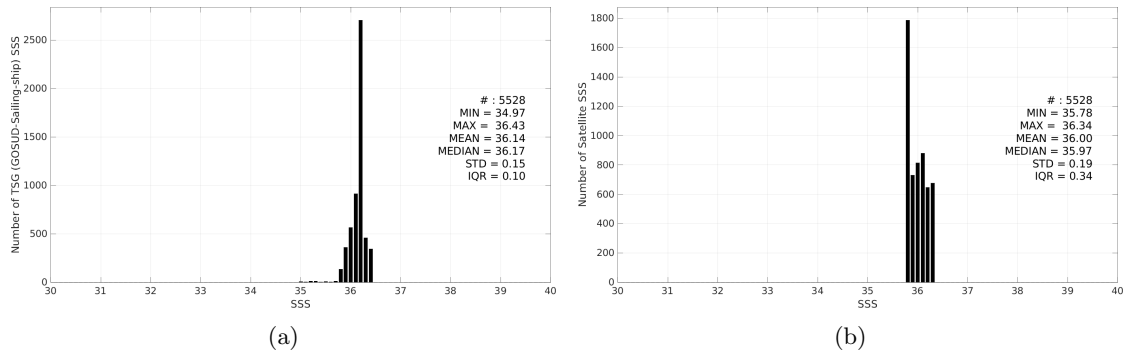
Figure 3: Histograms of SSS from TSG (GOSUD-Sailing-ship) (a) and SMOS SSS L3 v335 - Monthly - 25 km (CATDS-CPDC) (b) considering all match-up pairs per bins of 0.1 over the Gulf of Mexico Pi-MEP region and for the full satellite product period.
