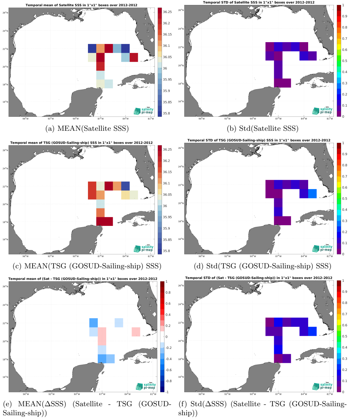
Figure 7: Temporal mean (left) and Std (right) of SSS from SMOS SSS L3 v335 - Monthly - 25 km (CATDS-CPDC) (top), TSG (GOSUD-Sailing-ship) (middle), and of \Delta SSS (Satellite - TSG (GOSUD-Sailing-ship)). Only match-up pairs are used to generate these maps.
