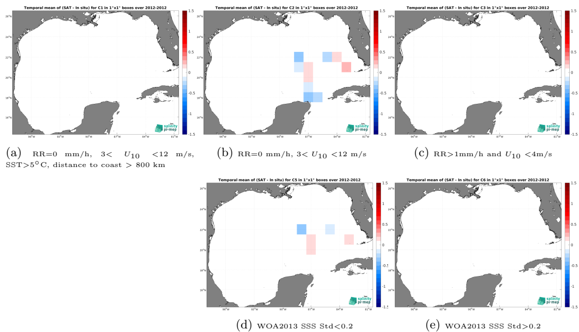
Figure 14: Temporal mean gridded over spatial boxes of size 1^\circ \times 1^\circ of \Delta\text{SSS} (SMOS SSS L3 v335 - Monthly - 25 km (CATDS-CPDC) - TSG (GOSUD-Sailing-ship)) for 5 different subdatasets corresponding to:RR=0 mm/h, 3 < U_{10} < 12 m/s, SST >5^\circ\text{C} , distance to coast > 800 km (a), RR=0 mm/h, 3 < U_{10} < 12 m/s (b), RR >1 mm/h and U_{10} < 4 m/s (c), WOA2013 SSS Std <0.2 (d), WOA2013 SSS Std >0.2 (e).
