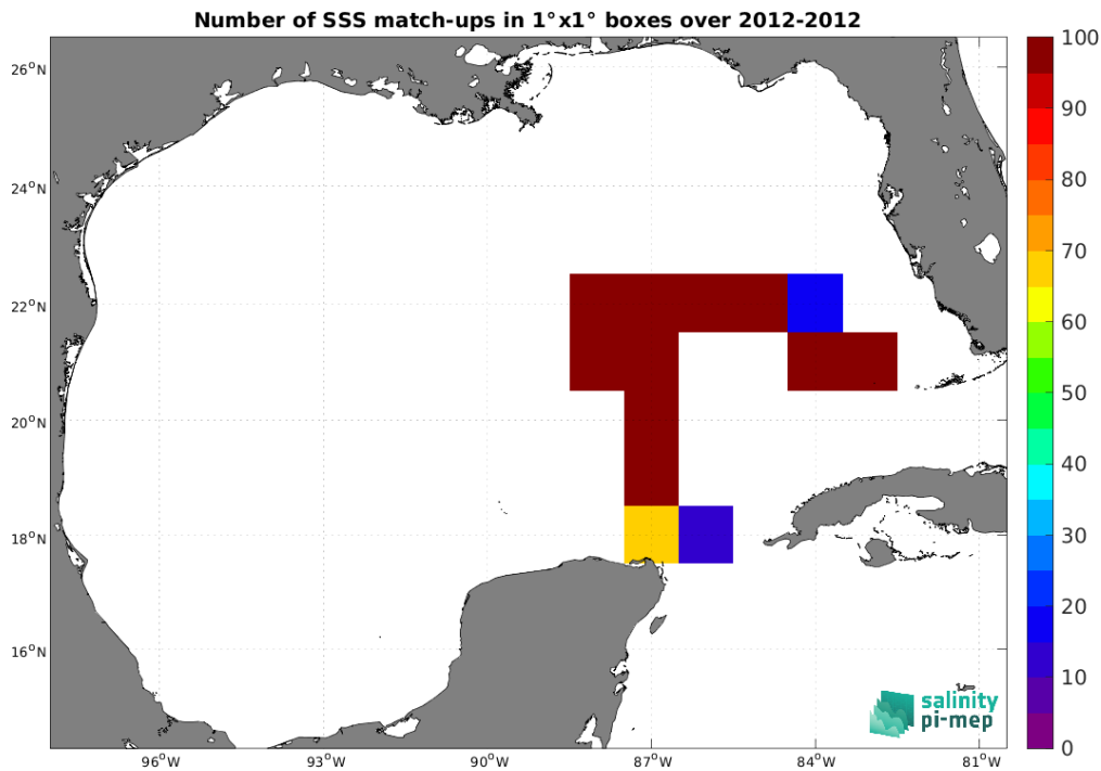
Figure 5: Number of SSS match-ups between TSG (GOSUD-Sailing-ship) SSS and the SMOS SSS L3 v335 - Monthly - 25 km (CATDS-CPDC) SSS product for the Gulf of Mexico Pi-MEP region over 1^\circ \times 1^\circ boxes and for the full satellite product period.
