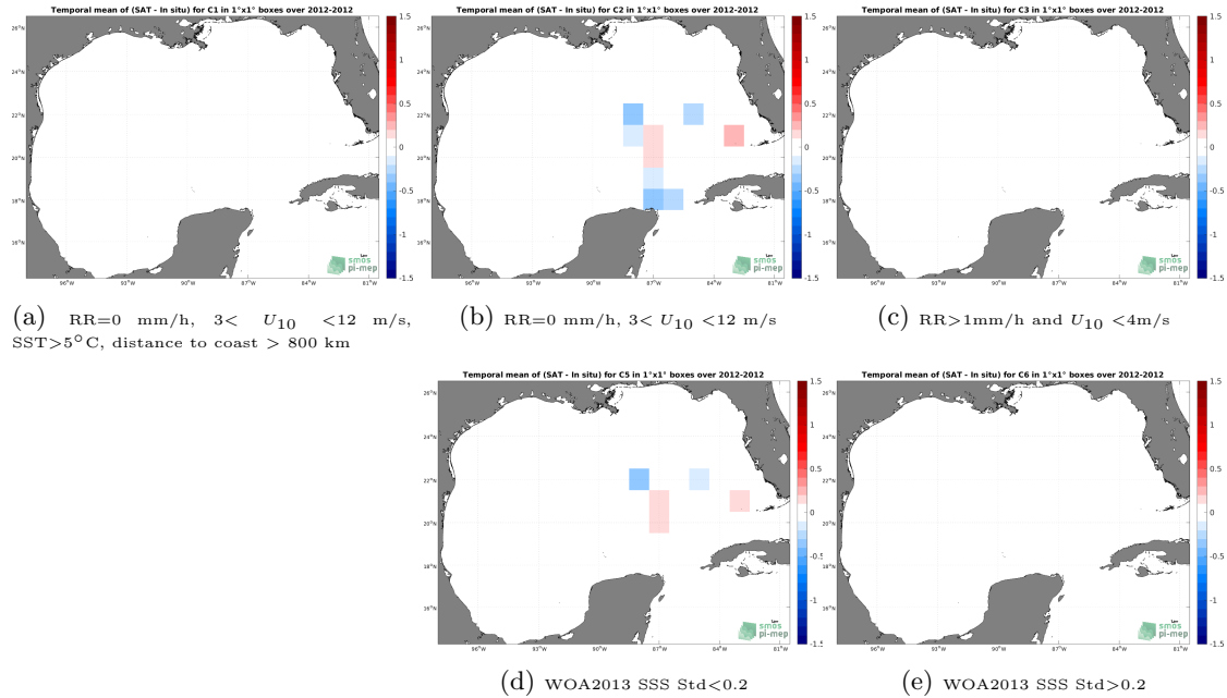
Figure 12: Temporal mean gridded over spatial boxes of size 1^{\circ}\times 1^{\circ} of \Delta SSS (SMOS SSS L3 v335 - Monthly - 25 km (CATDS-CPDC) - TSG (GOSUD-Sailing-ship)) for 5 different subdatasets corresponding to:RR=0 mm/h, 3 < U_{10} < 12 m/s, SST >5^{\circ}\text{C} , distance to coast > 800 km (a), RR=0 mm/h, 3 < U_{10} < 12 m/s (b), RR >1 mm/h and U_{10} < 4 m/s (c), WOA2013 SSS Std <0.2 (d), WOA2013 SSS Std >0.2 (e).
