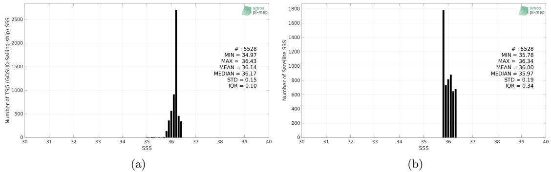
Figure 2: Histograms of SSS from TSG (GOSUD-Sailing-ship) (a) and SMOS SSS L3 v335 - Monthly - 25 km (CATDS-CPDC) (b) considering all match-up pairs per bins of 0.1 over the Gulf of Mexico Pi-MEP region and for the full satellite product period.
