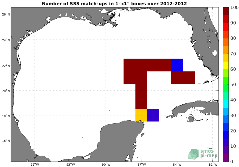
Figure 4: Number of SSS match-ups between TSG (GOSUD-Sailing-ship) SSS and the SMOS SSS L3 v335 - Monthly - 25 km (CATDS-CPDC) SSS product for the Gulf of Mexico Pi-MEP region over 1^\circ \times 1^\circ boxes and for the full satellite product period.
