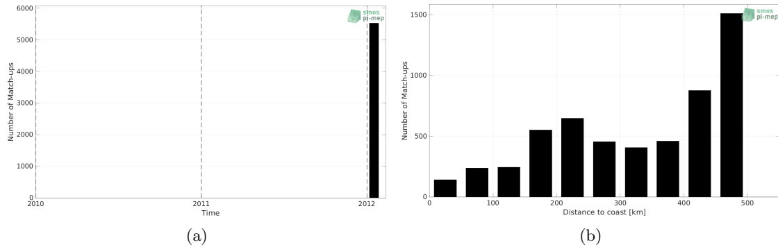
Figure 1: Number of match-ups between TSG (GOSUD-Sailing-ship) and SMOS SSS L3 v335 - Monthly - 25 km (CATDS-CPDC) SSS as a function of time (a) and as function of the distance to coast (b) over the Gulf of Mexico Pi-MEP region and for the full satellite product period.
