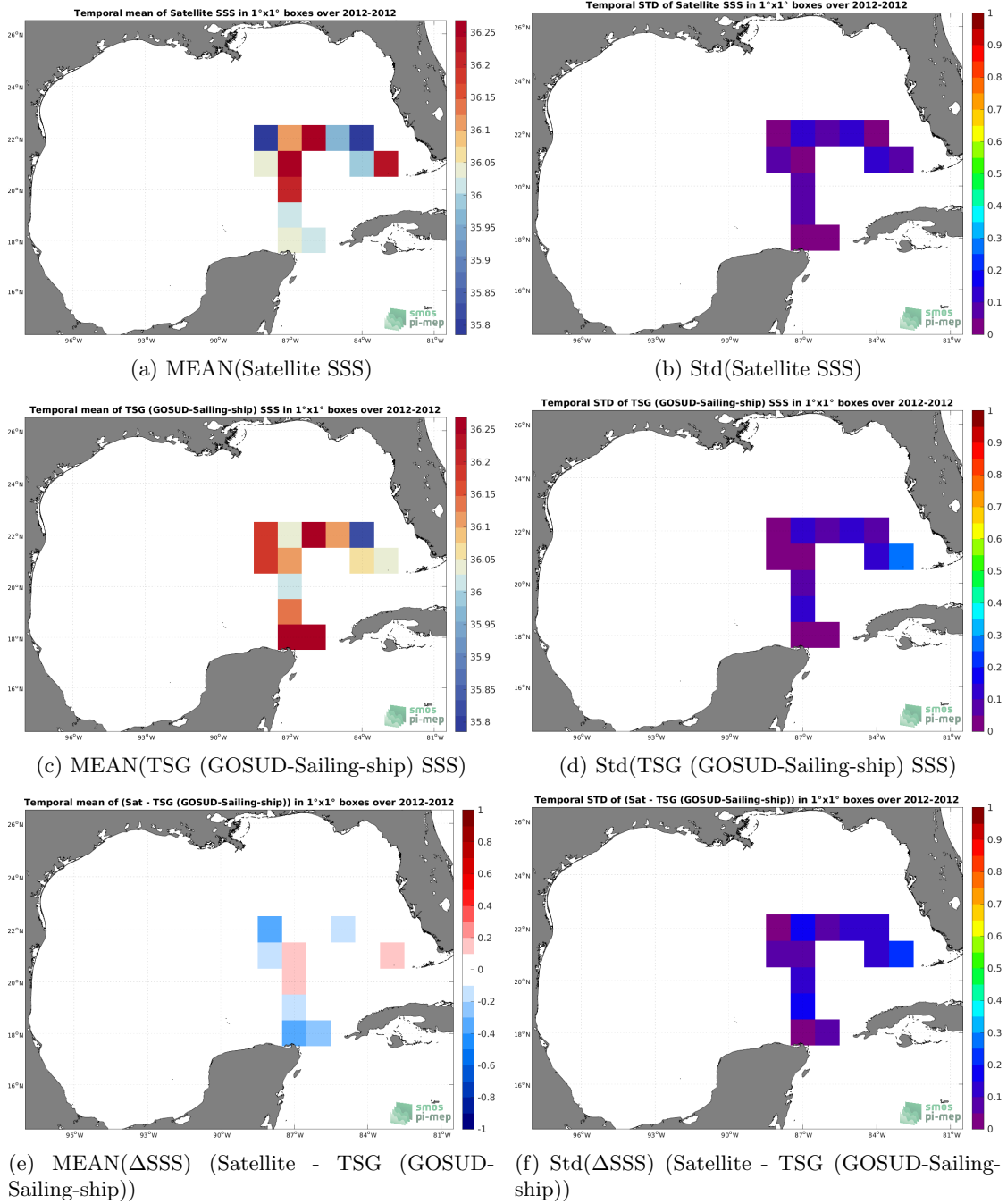
Figure 6: Temporal mean (left) and Std (right) of SSS from SMOS SSS L3 v335 - Monthly - 25 km (CATDS-CPDC) (top), TSG (GOSUD-Sailing-ship) (middle), and of \Delta SSS (Satellite - TSG (GOSUD-Sailing-ship)). Only match-up pairs are used to generate these maps.
