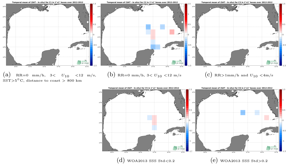
Figure 12: Temporal mean gridded over spatial boxes of size 1^\circ \times 1^\circ of \Delta SSS (SMOS SSS L3 v335 - Monthly - 25 km (CATDS-CPDC) - TSG (GOSUD-Sailing-ship)) for 5 different subdatasets corresponding to: RR=0 mm/h, 3 < U_{10} < 12 m/s, SST > 5^\circ\text{C} , distance to coast > 800 km (a), RR=0 mm/h, 3 < U_{10} < 12 m/s (b), RR > 1 mm/h and U_{10} < 4 m/s (c), WOA2013 SSS Std < 0.2 (d), WOA2013 SSS Std > 0.2 (e).
