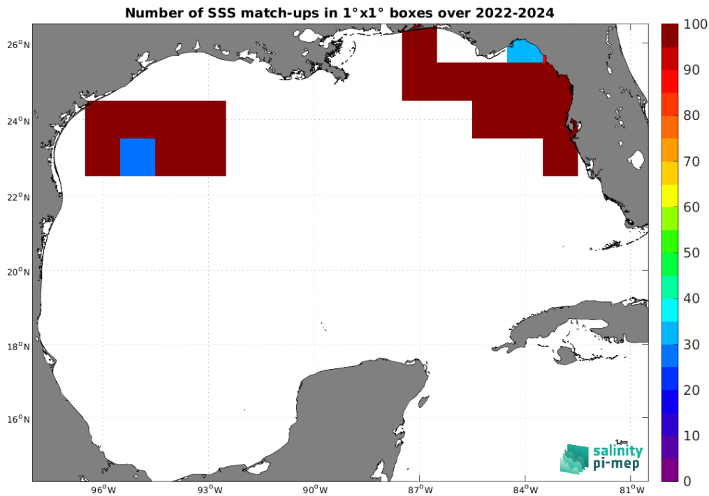
Figure 5: Number of SSS match-ups between Saildrone SSS and the SMOS SSS L3 v335 - Monthly - 25 km (CATDS-CPDC) SSS product for the Gulf of Mexico Pi-MEP region over 1^\circ \times 1^\circ boxes and for the full satellite product period.
