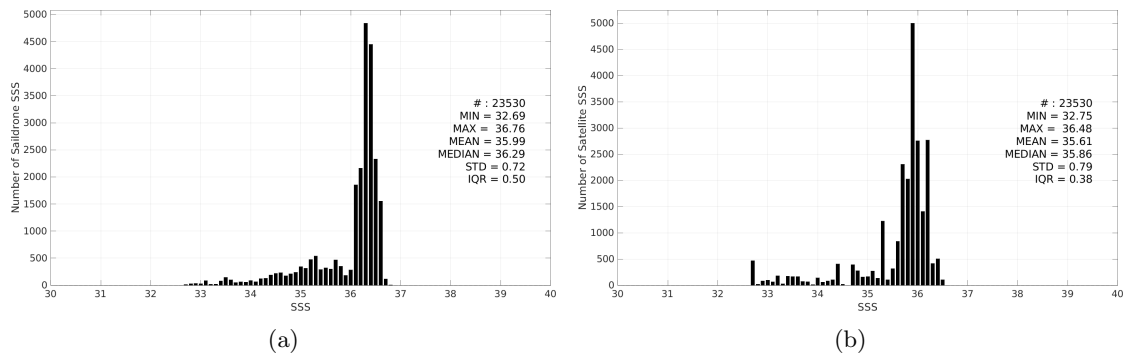
Figure 3: Histograms of SSS from Saildrone (a) and SMOS SSS L3 v335 - Monthly - 25 km (CATDS-CPDC) (b) considering all match-up pairs per bins of 0.1 over the Gulf of Mexico Pi-MEP region and for the full satellite product period.
