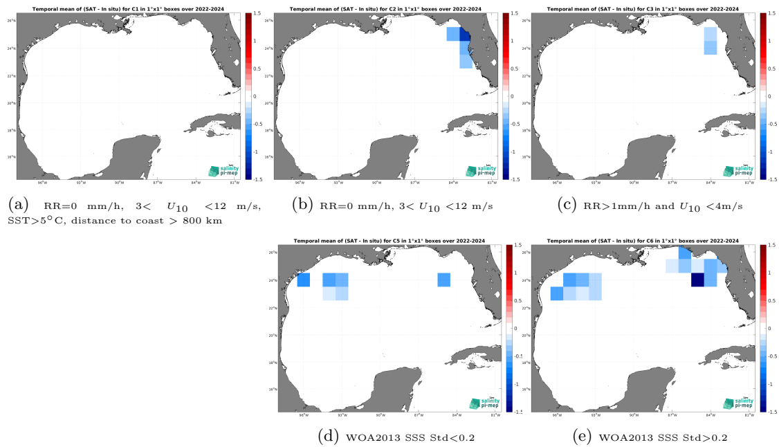
Figure 14: Temporal mean gridded over spatial boxes of size 1^\circ \times 1^\circ of \Delta SSS (SMOS SSS L3 v335 - Monthly - 25 km (CATDS-CPDC) - Saildrone) for 5 different subdatasets corresponding to:RR=0 mm/h, 3 < U_{10} < 12 m/s, SST >5^\circ C, distance to coast > 800 km (a), RR=0 mm/h, 3 < U_{10} < 12 m/s (b), RR >1 mm/h and U_{10} < 4 m/s (c), WOA2013 SSS Std <0.2 (d), WOA2013 SSS Std >0.2 (e).
