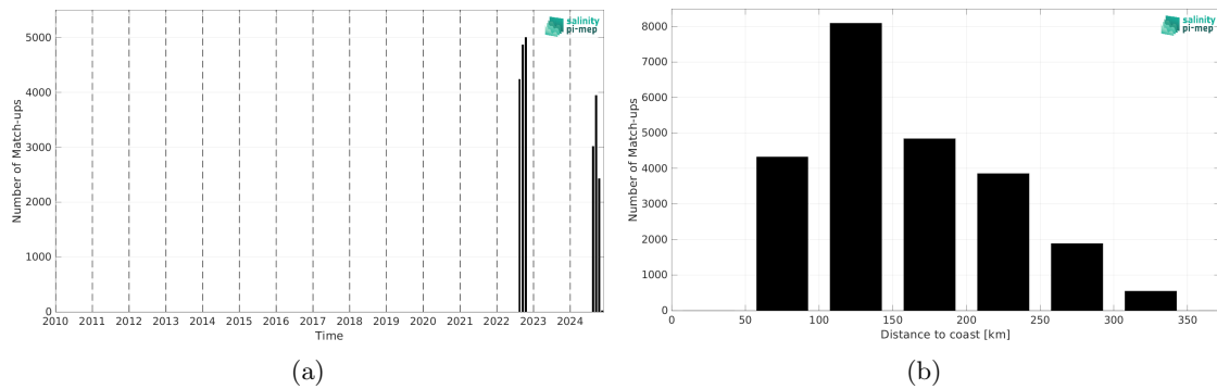
Figure 2: Number of match-ups between Saildrone and SMOS SSS L3 v335 - Monthly - 25 km (CATDS-CPDC) SSS as a function of time (a) and as function of the distance to coast (b) over the Gulf of Mexico Pi-MEP region and for the full satellite product period.
