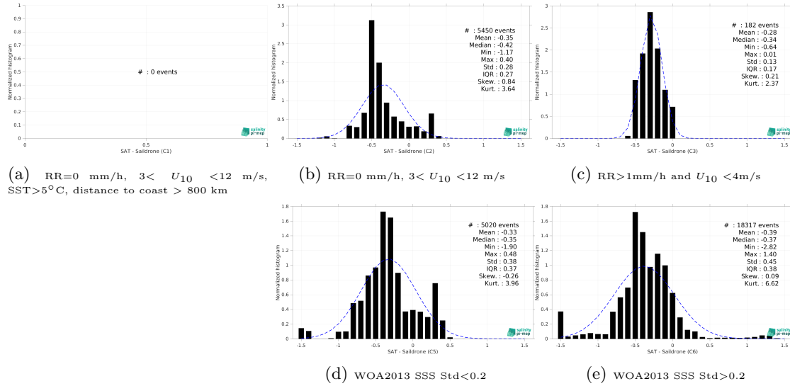
Figure 15: Normalized histogram of \Delta SSS (SMOS SSS L3 v335 - Monthly - 25 km (CATDS-CPDC) - Salldrone) for 5 different subdatasets corresponding to: RR=0 mm/h, 3 < U_{10} < 12 m/s, SST > 5°C, distance to coast > 800 km (a), RR=0 mm/h, 3 < U_{10} < 12 m/s (b), RR > 1mm/h and U_{10} < 4 m/s (c), WOA2013 SSS Std < 0.2 (d), WOA2013 SSS Std > 0.2 (e).
