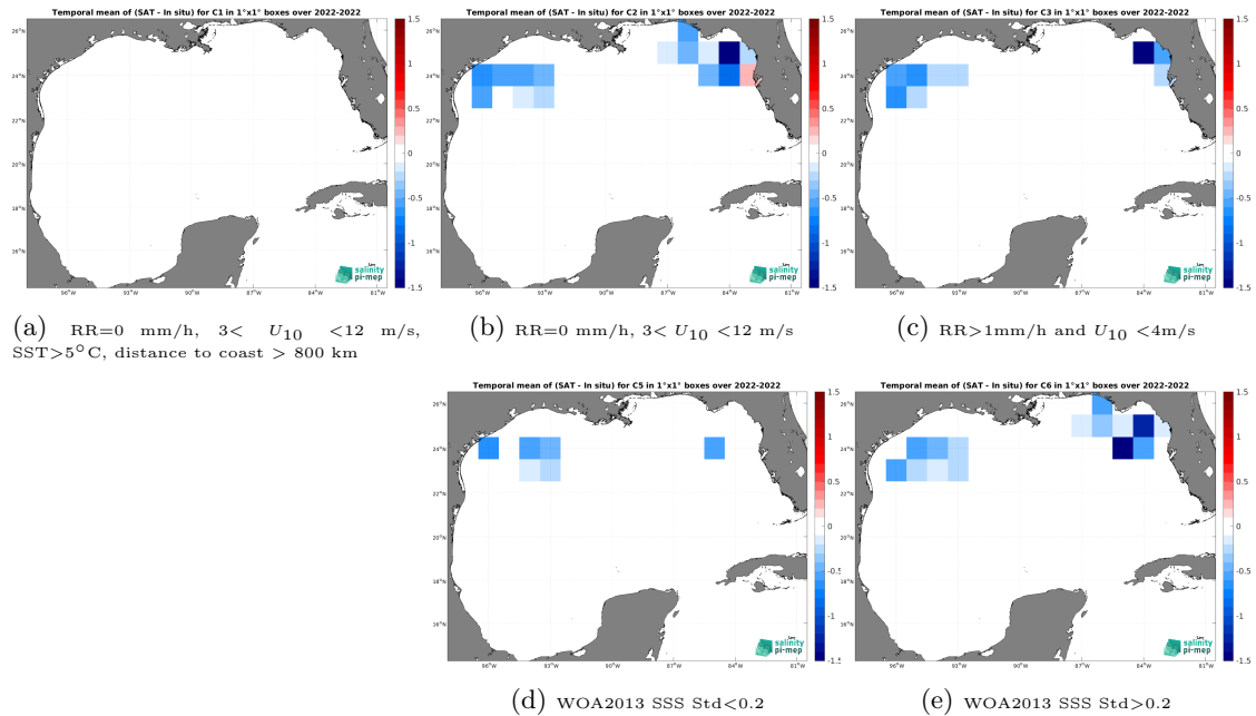
Figure 12: Temporal mean gridded over spatial boxes of size 1^{\circ}\times 1^{\circ} of \Delta\text{SSS} (SMOS SSS L3 v335 - Monthly - 25 km (CATDS-CPDC) - Saildrone) for 5 different subdatasets corresponding to:RR=0 mm/h, 3 < U_{10} < 12 m/s, SST >5^{\circ}\text{C} , distance to coast > 800 km (a), RR=0 mm/h, 3 < U_{10} < 12 m/s (b), RR >1 mm/h and U_{10} < 4 m/s (c), WOA2013 SSS Std <0.2 (d), WOA2013 SSS Std >0.2 (e).
