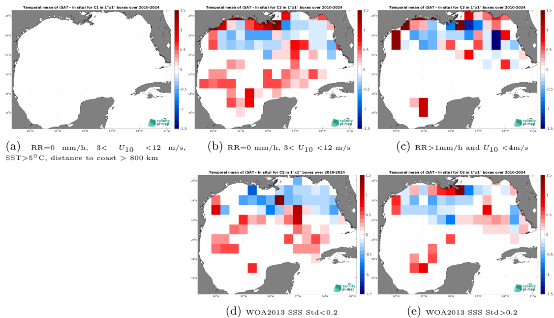
Figure 14: Temporal mean gridded over spatial boxes of size 1^\circ \times 1^\circ of \Delta\text{SSS} (SMOS SSS L3 v335 - 10 Days - 25 km (CATDS-CPDC) - TSG (SAMOS)) for 5 different subdatasets corresponding to:RR=0 mm/h, 3 < U_{10} < 12 m/s, SST >5^\circ\text{C} , distance to coast > 800 km (a), RR=0 mm/h, 3 < U_{10} < 12 m/s (b), RR >1 mm/h and U_{10} < 4 m/s (c), WOA2013 SSS Std <0.2 (d), WOA2013 SSS Std >0.2 (e).
