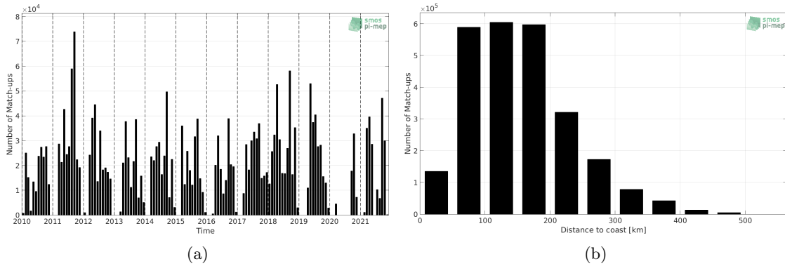
Figure 1: Number of match-ups between TSG (SAMOS) and SMOS SSS L3 v335 - 10 Days - 25 km (CATDS-CPDC) SSS as a function of time (a) and as function of the distance to coast (b) over the Gulf of Mexico Pi-MEP region and for the full satellite product period.
