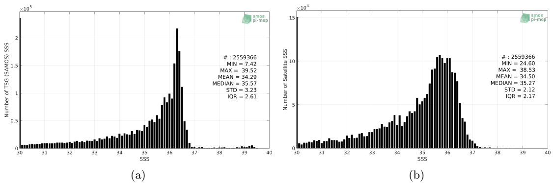
Figure 2: Histograms of SSS from TSG (SAMOS) (a) and SMOS SSS L3 v335 - 10 Days - 25 km (CATDS-CPDC) (b) considering all match-up pairs per bins of 0.1 over the Gulf of Mexico Pi-MEP region and for the full satellite product period.
