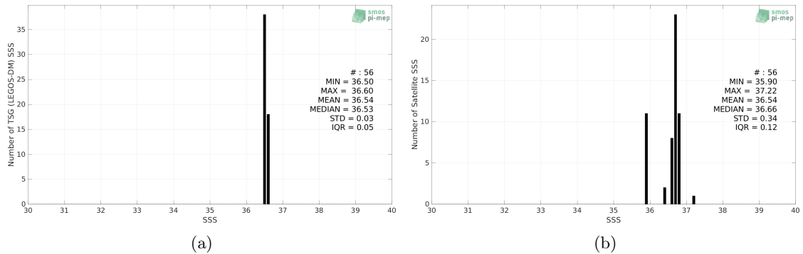
Figure 2: Histograms of SSS from TSG (LEGOS-DM) (a) and SMOS SSS L3 v335 - 10 Days - 25 km (CATDS-CPDC) (b) considering all match-up pairs per bins of 0.1 over the Gulf of Mexico Pi-MEP region and for the full satellite product period.
