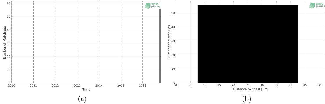
Figure 1: Number of match-ups between TSG (LEGOS-DM) and SMOS SSS L3 v335 - 10 Days - 25 km (CATDS-CPDC) SSS as a function of time (a) and as function of the distance to coast (b) over the Gulf of Mexico Pi-MEP region and for the full satellite product period.
