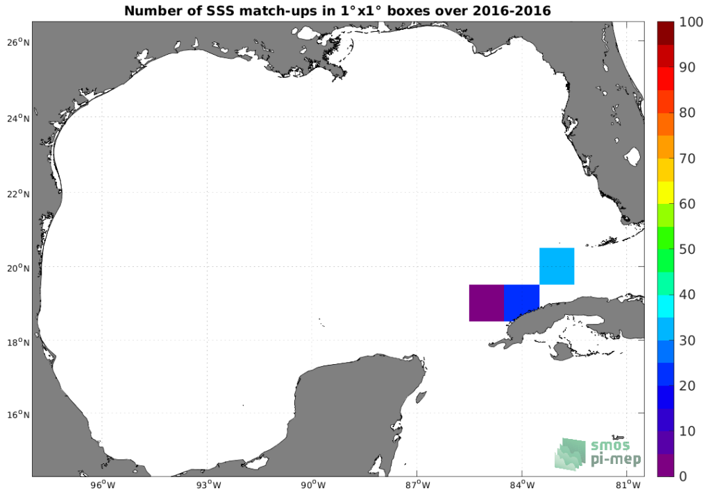
Figure 4: Number of SSS match-ups between TSG (LEGOS-DM) SSS and the SMOS SSS L3 v335 - 10 Days - 25 km (CATDS-CPDC) SSS product for the Gulf of Mexico Pi-MEP region over 1^\circ \times 1^\circ boxes and for the full satellite product period.
