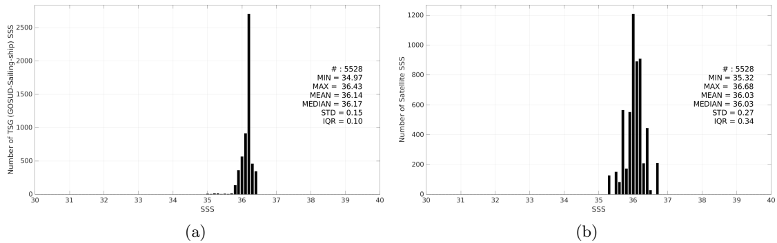
Figure 3: Histograms of SSS from TSG (GOSUD-Sailing-ship) (a) and SMOS SSS L3 v335 - 10 Days - 25 km (CATDS-CPDC) (b) considering all match-up pairs per bins of 0.1 over the Gulf of Mexico Pi-MEP region and for the full satellite product period.
