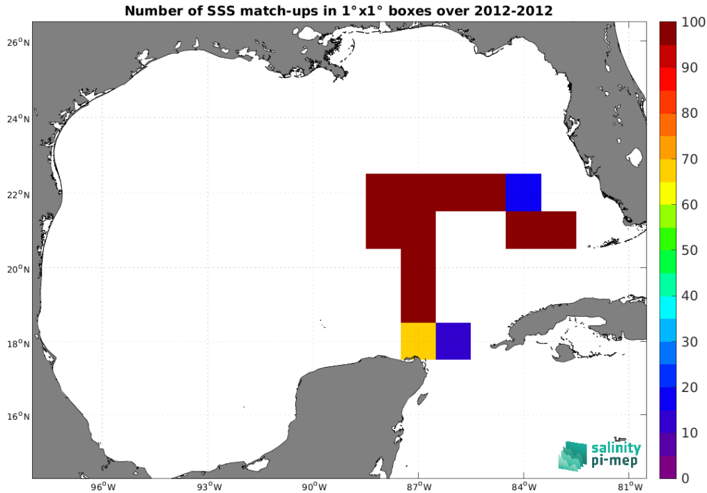
Figure 5: Number of SSS match-ups between TSG (GOSUD-Sailing-ship) SSS and the SMOS SSS L3 v335 - 10 Days - 25 km (CATDS-CPDC) SSS product for the Gulf of Mexico Pi-MEP region over 1^\circ \times 1^\circ boxes and for the full satellite product period.
