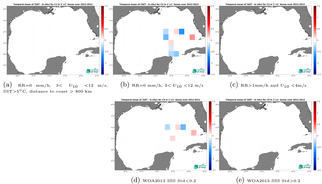
Figure 14: Temporal mean gridded over spatial boxes of size 1^\circ \times 1^\circ of \Delta\text{SSS} (SMOS SSS L3 v335 - 10 Days - 25 km (CATDS-CPDC) - TSG (GOSUD-Sailing-ship)) for 5 different subdatasets corresponding to:RR=0 mm/h, 3 < U_{10} < 12 m/s, SST >5^\circ\text{C} , distance to coast > 800 km (a), RR=0 mm/h, 3 < U_{10} < 12 m/s (b), RR >1 mm/h and U_{10} < 4 m/s (c), WOA2013 SSS Std <0.2 (d), WOA2013 SSS Std >0.2 (e).
