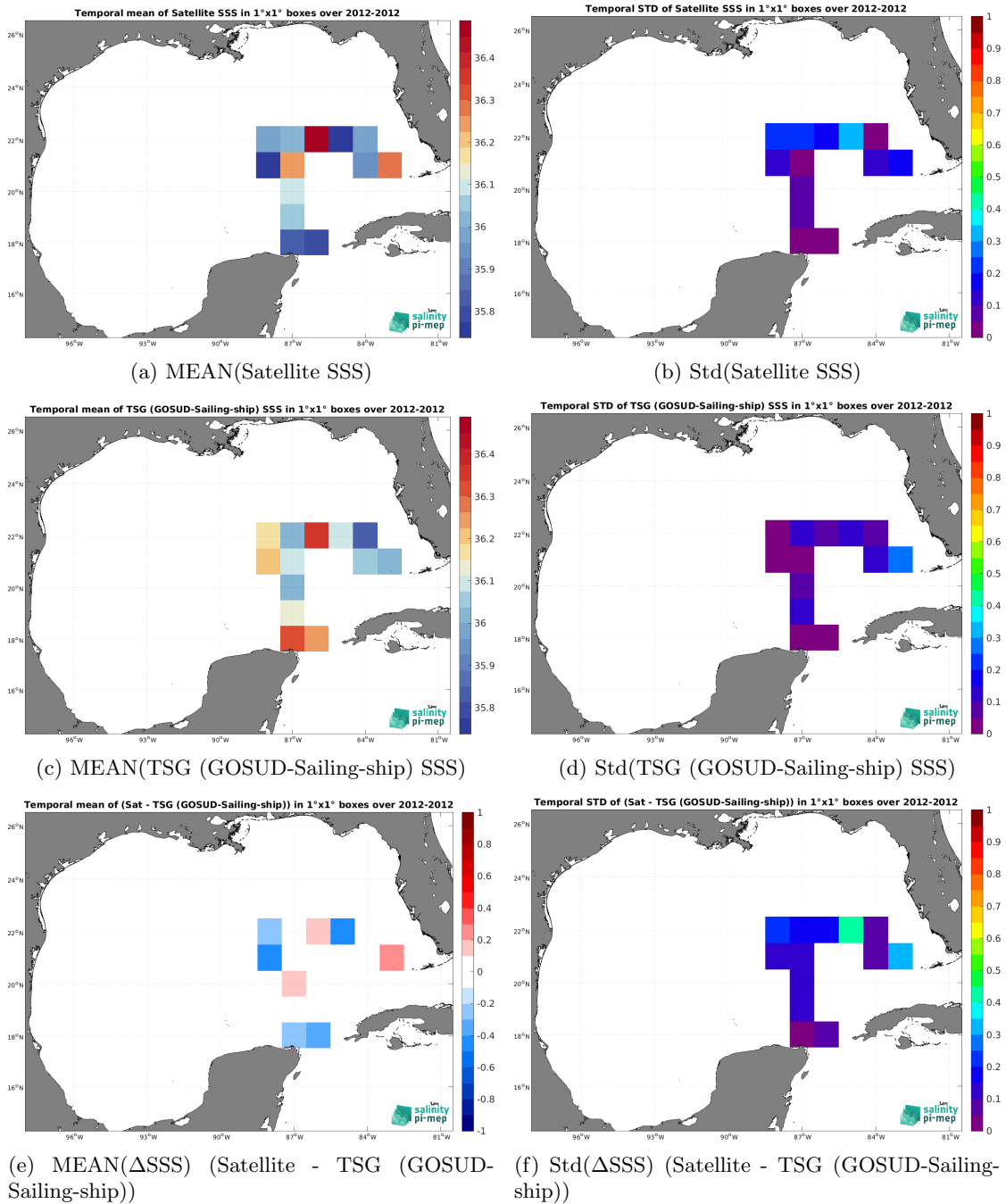
Figure 7: Temporal mean (left) and Std (right) of SSS from SMOS SSS L3 v335 - 10 Days - 25 km (CATDS-CPDC) (top), TSG (GOSUD-Sailing-ship) (middle), and of \Delta SSS (Satellite - TSG (GOSUD-Sailing-ship)). Only match-up pairs are used to generate these maps.
