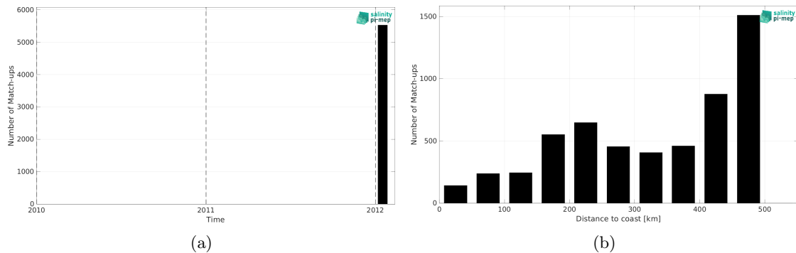
Figure 2: Number of match-ups between TSG (GOSUD-Sailing-ship) and SMOS SSS L3 v335 - 10 Days - 25 km (CATDS-CPDC) SSS as a function of time (a) and as function of the distance to coast (b) over the Gulf of Mexico Pi-MEP region and for the full satellite product period.
