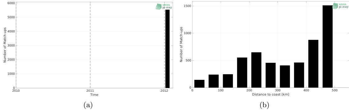
Figure 1: Number of match-ups between TSG (GOSUD-Sailing-ship) and SMOS SSS L3 v335 - 10 Days - 25 km (CATDS-CPDC) SSS as a function of time (a) and as function of the distance to coast (b) over the Gulf of Mexico Pi-MEP region and for the full satellite product period.
