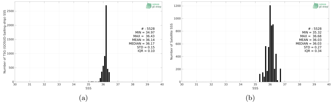
Figure 2: Histograms of SSS from TSG (GOSUD-Sailing-ship) (a) and SMOS SSS L3 v335 - 10 Days - 25 km (CATDS-CPDC) (b) considering all match-up pairs per bins of 0.1 over the Gulf of Mexico Pi-MEP region and for the full satellite product period.
