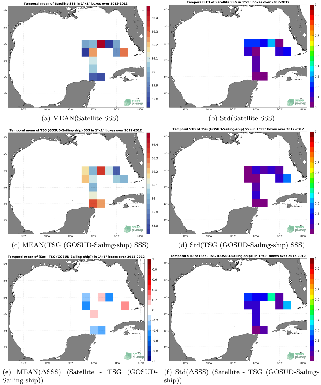
Figure 6: Temporal mean (left) and Std (right) of SSS from SMOS SSS L3 v335 - 10 Days - 25 km (CATDS-CPDC) (top), TSG (GOSUD-Sailing-ship) (middle), and of \Delta SSS (Satellite - TSG (GOSUD-Sailing-ship)). Only match-up pairs are used to generate these maps.
