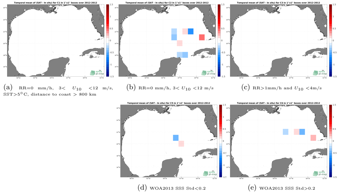
Figure 12: Temporal mean gridded over spatial boxes of size 1^\circ \times 1^\circ of \Delta SSS (SMOS SSS L3 v335 - 10 Days - 25 km (CATDS-CPDC) - TSG (GOSUD-Sailing-ship)) for 5 different subdatasets corresponding to:RR=0 mm/h, 3 < U_{10} < 12 m/s, SST >5^\circ\text{C} , distance to coast > 800 km (a), RR=0 mm/h, 3 < U_{10} < 12 m/s (b), RR >1 mm/h and U_{10} < 4 m/s (c), WOA2013 SSS Std <0.2 (d), WOA2013 SSS Std >0.2 (e).
