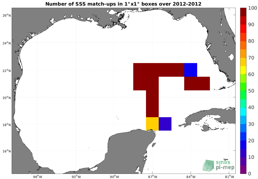
Figure 4: Number of SSS match-ups between TSG (GOSUD-Sailing-ship) SSS and the SMOS SSS L3 v335 - 10 Days - 25 km (CATDS-CPDC) SSS product for the Gulf of Mexico Pi-MEP region over 1^\circ \times 1^\circ boxes and for the full satellite product period.
