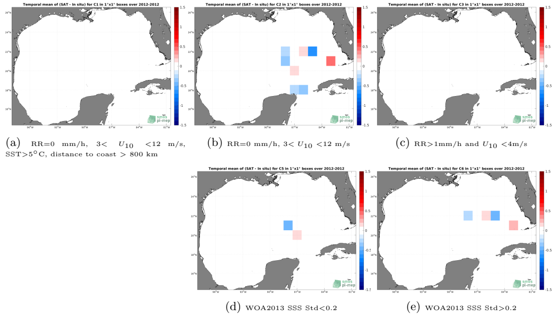
Figure 12: Temporal mean gridded over spatial boxes of size 1^{\circ}\times 1^{\circ} of \Delta SSS (SMOS SSS L3 v335 - 10 Days - 25 km (CATDS-CPDC) - TSG (GOSUD-Sailing-ship)) for 5 different subdatasets corresponding to:RR=0 mm/h, 3 < U_{10} < 12 m/s, SST >5^{\circ}\text{C} , distance to coast > 800 km (a), RR=0 mm/h, 3 < U_{10} < 12 m/s (b), RR >1 mm/h and U_{10} < 4 m/s (c), WOA2013 SSS Std <0.2 (d), WOA2013 SSS Std >0.2 (e).
