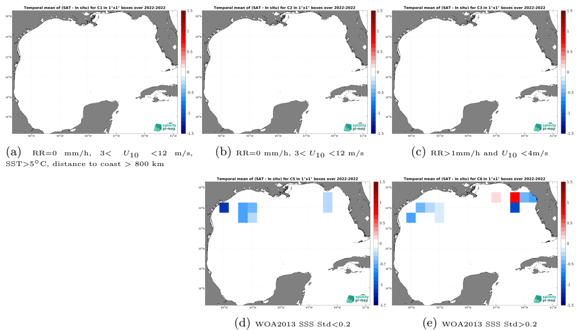
Figure 14: Temporal mean gridded over spatial boxes of size 1^\circ \times 1^\circ of \Delta SSS (SMOS SSS L3 v335 - 10 Days - 25 km (CATDS-CPDC) - Saildrone) for 5 different subdatasets corresponding to:RR=0 mm/h, 3 < U_{10} < 12 m/s, SST>5°C, distance to coast > 800 km (a), RR=0 mm/h, 3 < U_{10} < 12 m/s (b), RR>1mm/h and U_{10} < 4 m/s (c), WOA2013 SSS Std<0.2 (d), WOA2013 SSS Std>0.2 (e).
