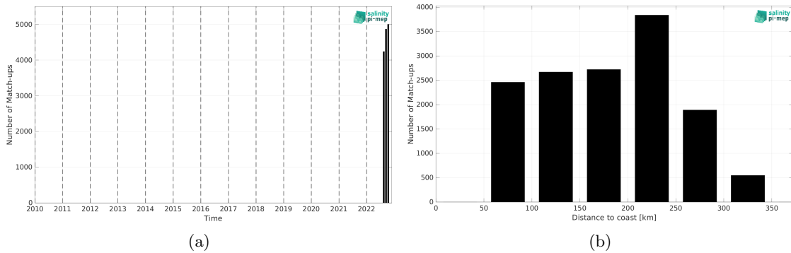
Figure 2: Number of match-ups between Saildrone and SMOS SSS L3 v335 - 10 Days - 25 km (CATDS-CPDC) SSS as a function of time (a) and as function of the distance to coast (b) over the Gulf of Mexico Pi-MEP region and for the full satellite product period.
