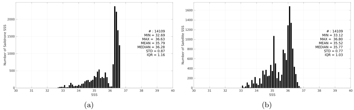
Figure 3: Histograms of SSS from Saildrone (a) and SMOS SSS L3 v335 - 10 Days - 25 km (CATDS-CPDC) (b) considering all match-up pairs per bins of 0.1 over the Gulf of Mexico Pi-MEP region and for the full satellite product period.
