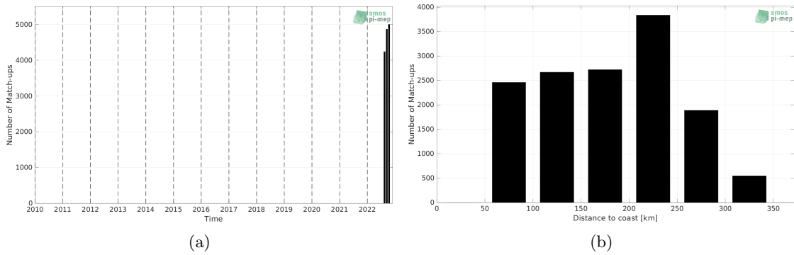
Figure 1: Number of match-ups between Saildrone and SMOS SSS L3 v335 - 10 Days - 25 km (CATDS-CPDC) SSS as a function of time (a) and as function of the distance to coast (b) over the Gulf of Mexico Pi-MEP region and for the full satellite product period.
