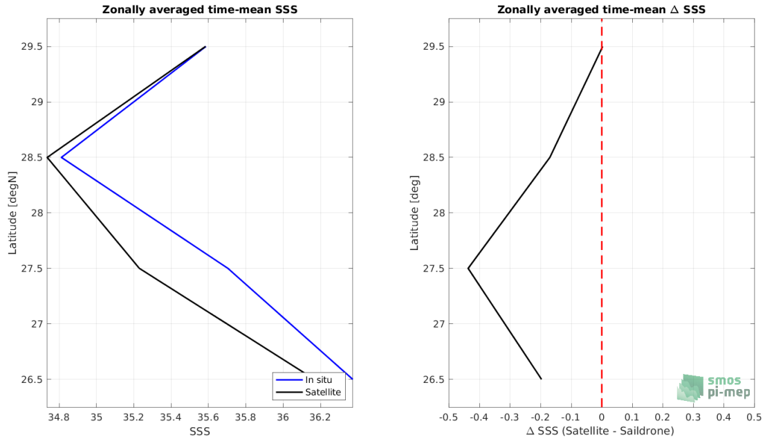
Figure 8: Left panel: Zonal mean SSS from SMOS SSS L3 v335 - 10 Days - 25 km (CATDS-CPDC) satellite product (black) and from Sailldrone (blue). Right panel: Zonal mean of \Delta SSS (Satellite - Sailldrone) for all the collected Pi-MEP match-up pairs estimated over the full satellite product period.
