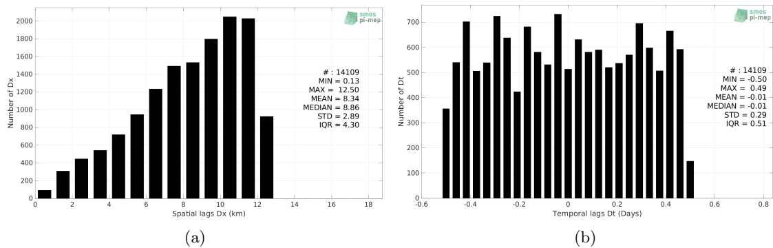
Figure 5: Histograms of the spatial (a) and temporal (b) lags between the location/time of the Sailldrone measurement and the date of the corresponding SMOS SSS L3 v335 - 10 Days - 25 km (CATDS-CPDC) SSS pixel.
