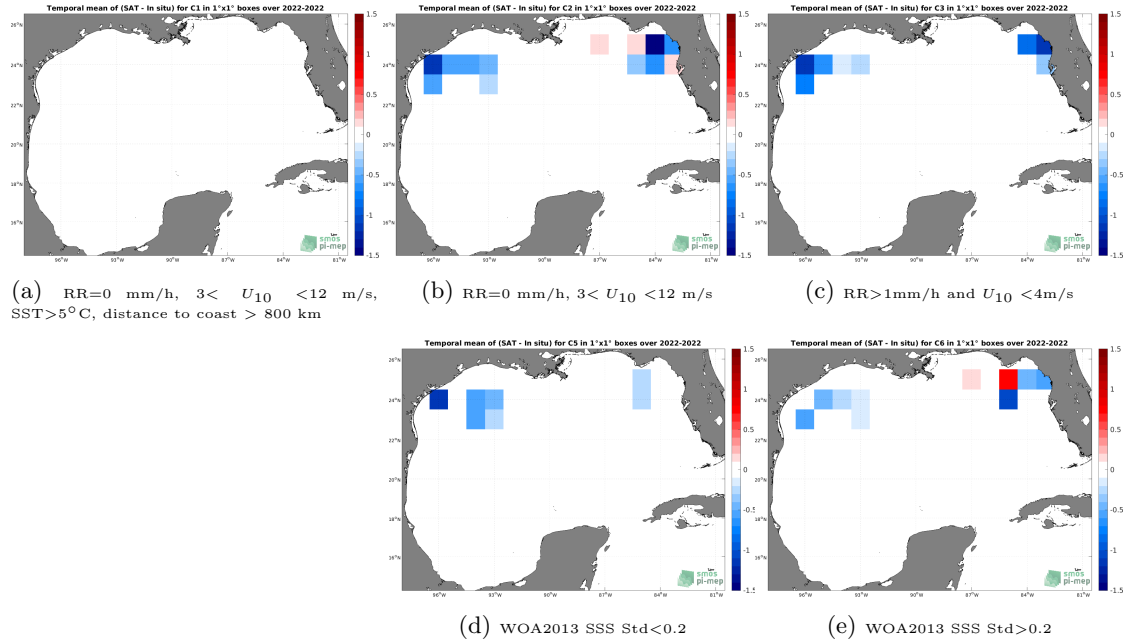
Figure 12: Temporal mean gridded over spatial boxes of size 1^{\circ}\times 1^{\circ} of \Delta\text{SSS} (SMOS SSS L3 v335 - 10 Days - 25 km (CATDS-CPDC) - Saildrone) for 5 different subdatasets corresponding to:RR=0 mm/h, 3 < U_{10} < 12 m/s, SST >5^{\circ}\text{C} , distance to coast > 800 km (a), RR=0 mm/h, 3 < U_{10} < 12 m/s (b), RR >1 mm/h and U_{10} < 4 m/s (c), WOA2013 SSS Std <0.2 (d), WOA2013 SSS Std >0.2 (e).
