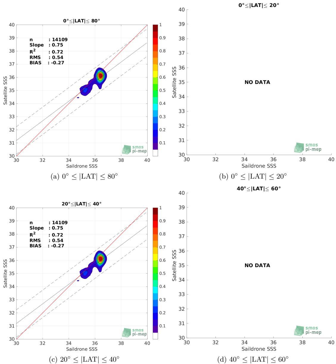
Figure 9: Contour maps of the concentration of SMOS SSS L3 v335 - 10 Days - 25 km (CATDS-CPDC) SSS (y-axis) versus Saïldrone SSS (x-axis) at match-up pairs for different latitude bands. For each plot, the red line shows x=y . The black thin and dashed lines indicate a linear fit through the data cloud and the \pm 95\% confidence levels, respectively. The number match-up pairs n , the slope and R^2 coefficient of the linear fit, the root mean square (RMS) and the mean bias between satellite and in situ data are indicated for each latitude band in each plots.
