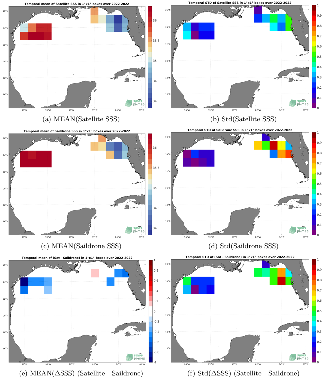
Figure 6: Temporal mean (left) and Std (right) of SSS from SMOS SSS L3 v335 - 10 Days - 25 km (CATDS-CPDC) (top), Saildrone (middle), and of \Delta SSS (Satellite - Saildrone). Only match-up pairs are used to generate these maps.
