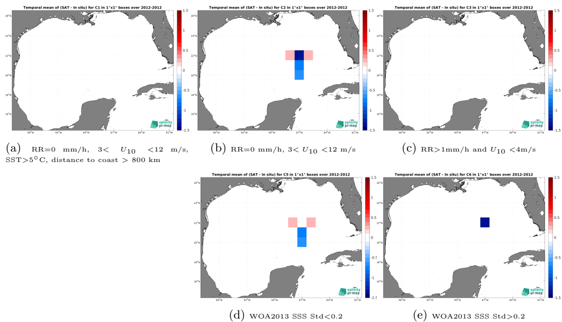
Figure 14: Temporal mean gridded over spatial boxes of size 1^\circ \times 1^\circ of \Delta\text{SSS} (SMOS SSS L2Q v333 - 0.25 Deg (CATDS-CPDC) - TSG (GOSUD-Sailing-ship)) for 5 different subdatasets corresponding to: RR=0 mm/h, 3 < U_{10} < 12 m/s, SST > 5°C, distance to coast > 800 km (a), RR=0 mm/h, 3 < U_{10} < 12 m/s (b), RR > 1mm/h and U_{10} < 4 m/s (c), WOA2013 SSS Std < 0.2 (d), WOA2013 SSS Std > 0.2 (e).
