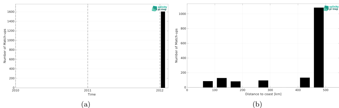
Figure 2: Number of match-ups between TSG (GOSUD-Sailing-ship) and SMOS SSS L2Q v333 - 0.25 Deg (CATDS-CPDC) SSS as a function of time (a) and as function of the distance to coast (b) over the Gulf of Mexico Pi-MEP region and for the full satellite product period.
