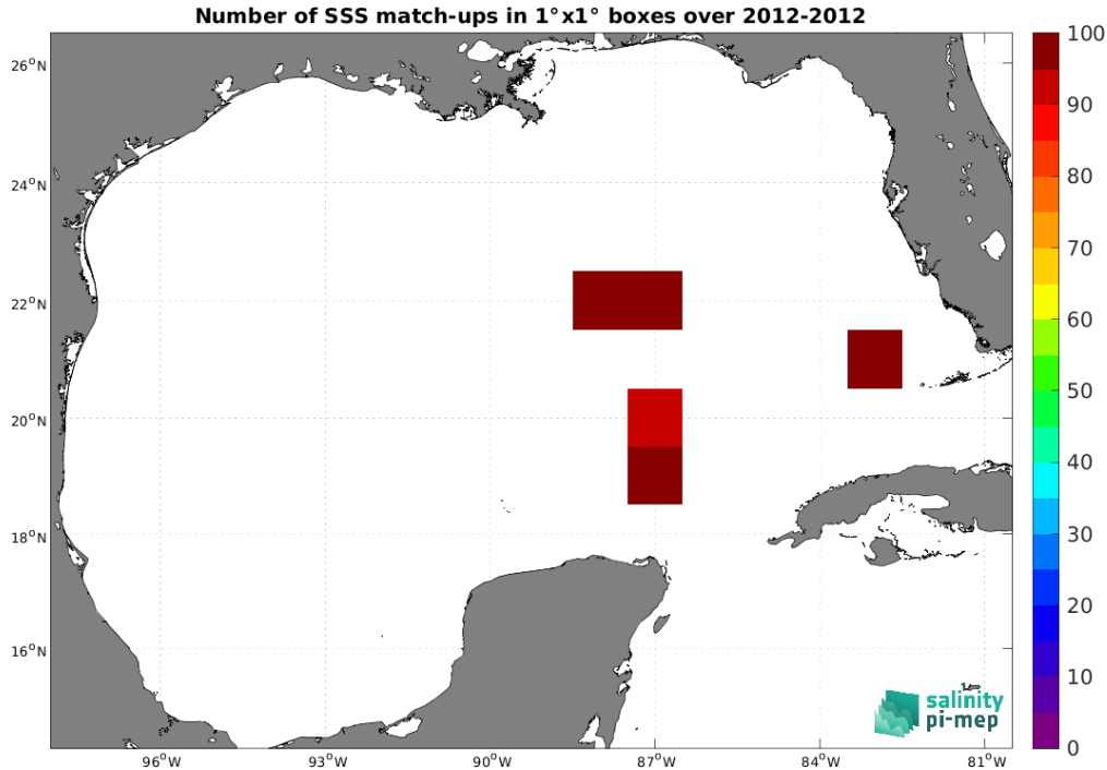
Figure 5: Number of SSS match-ups between TSG (GOSUD-Sailing-ship) SSS and the SMOS SSS L2Q v333 - 0.25 Deg (CATDS-CPDC) SSS product for the Gulf of Mexico Pi-MEP region over 1^\circ \times 1^\circ boxes and for the full satellite product period.
