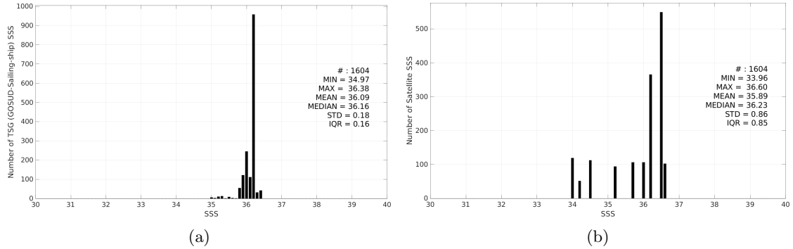
Figure 3: Histograms of SSS from TSG (GOSUD-Sailing-ship) (a) and SMOS SSS L2Q v333 - 0.25 Deg (CATDS-CPDC) (b) considering all match-up pairs per bins of 0.1 over the Gulf of Mexico Pi-MEP region and for the full satellite product period.
