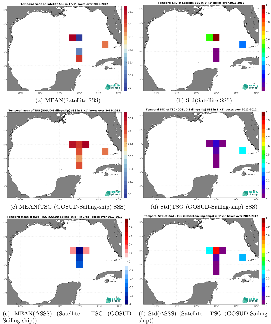
Figure 7: Temporal mean (left) and Std (right) of SSS from SMOS SSS L2Q v333 - 0.25 Deg (CATDS-CPDC) (top), TSG (GOSUD-Sailing-ship) (middle), and of \Delta SSS (Satellite - TSG (GOSUD-Sailing-ship)). Only match-up pairs are used to generate these maps.
