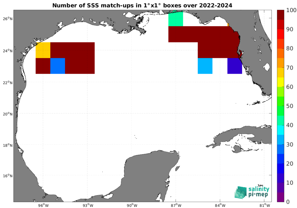
Figure 5: Number of SSS match-ups between Saildrone SSS and the SMOS SSS L2Q v333 - 0.25 Deg (CATDS-CPDC) SSS product for the Gulf of Mexico Pi-MEP region over 1°×1° boxes and for the full satellite product period.
