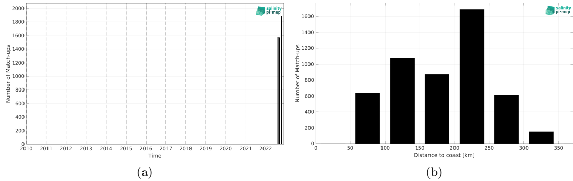
Figure 2: Number of match-ups between Saildrone and SMOS SSS L2Q v333 - 0.25 Deg (CATDS-CPDC) SSS as a function of time (a) and as function of the distance to coast (b) over the Gulf of Mexico Pi-MEP region and for the full satellite product period.
