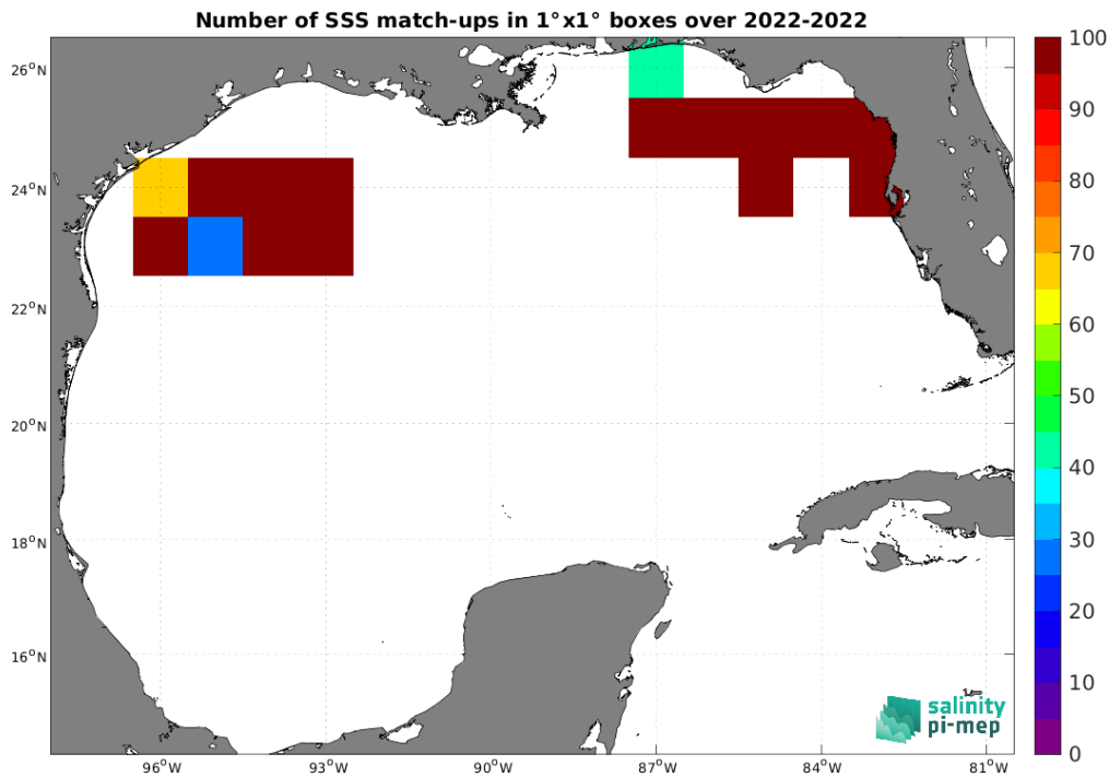
Figure 5: Number of SSS match-ups between Saildrone SSS and the SMOS SSS L2Q v333 - 0.25 Deg (CATDS-CPDC) SSS product for the Gulf of Mexico Pi-MEP region over 1^\circ \times 1^\circ boxes and for the full satellite product period.
