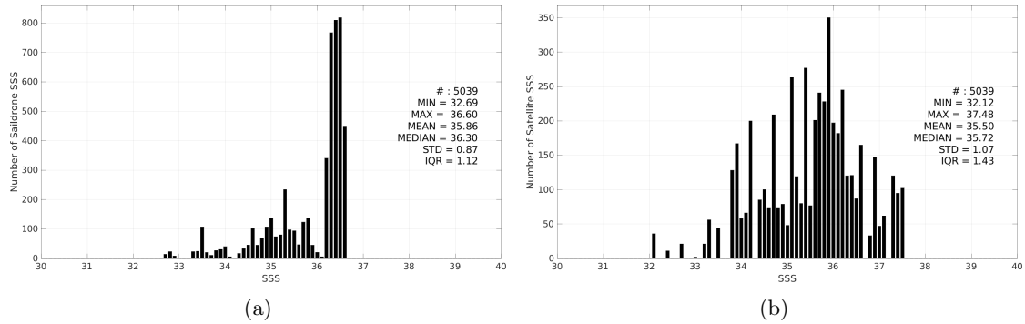
Figure 3: Histograms of SSS from Saildrone (a) and SMOS SSS L2Q v333 - 0.25 Deg (CATDS-CPDC) (b) considering all match-up pairs per bins of 0.1 over the Gulf of Mexico Pi-MEP region and for the full satellite product period.
