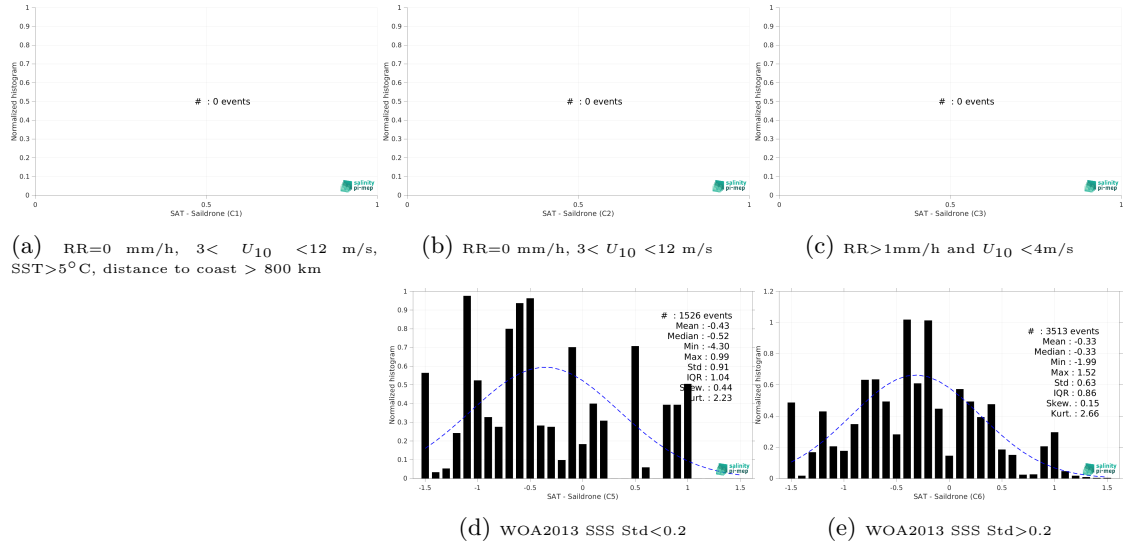
Figure 15: Normalized histogram of \Delta SSS (SMOS SSS L2Q v333 - 0.25 Deg (CATDS-CPDC) - Salldrone) for 5 different subdatasets corresponding to: RR=0 mm/h, 3 < U_{10} < 12 m/s, SST>5°C, distance to coast > 800 km (a), RR=0 mm/h, 3 < U_{10} < 12 m/s (b), RR>1mm/h and U_{10} < 4 m/s (c), WOA2013 SSS Std<0.2 (d), WOA2013 SSS Std>0.2 (e).
