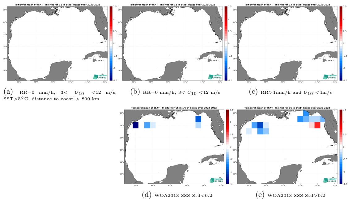
Figure 14: Temporal mean gridded over spatial boxes of size 1^\circ \times 1^\circ of \Delta\text{SSS} (SMOS SSS L2Q v333 - 0.25 Deg (CATDS-CPDC) - Saildrone) for 5 different subdatasets corresponding to: RR=0 mm/h, 3 < U_{10} < 12 m/s, SST > 5°C, distance to coast > 800 km (a), RR=0 mm/h, 3 < U_{10} < 12 m/s (b), RR > 1mm/h and U_{10} < 4 m/s (c), WOA2013 SSS Std < 0.2 (d), WOA2013 SSS Std > 0.2 (e).
