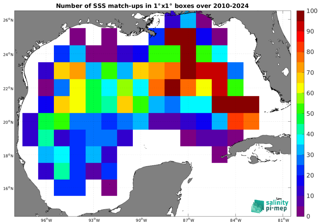
Figure 5: Number of SSS match-ups between Argo SSS and the SMOS SSS L2Q v333 - 0.25 Deg (CATDS-CPDC) SSS product for the Gulf of Mexico Pi-MEP region over 1^\circ \times 1^\circ boxes and for the full satellite product period.
