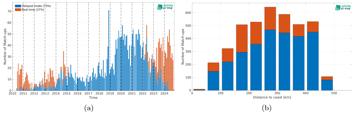
Figure 2: Number of match-ups between Argo and SMOS SSS L2Q v333 - 0.25 Deg (CATDS-CPDC) SSS as a function of time (a) and as function of the distance to coast (b) over the Gulf of Mexico Pi-MEP region and for the full satellite product period.
