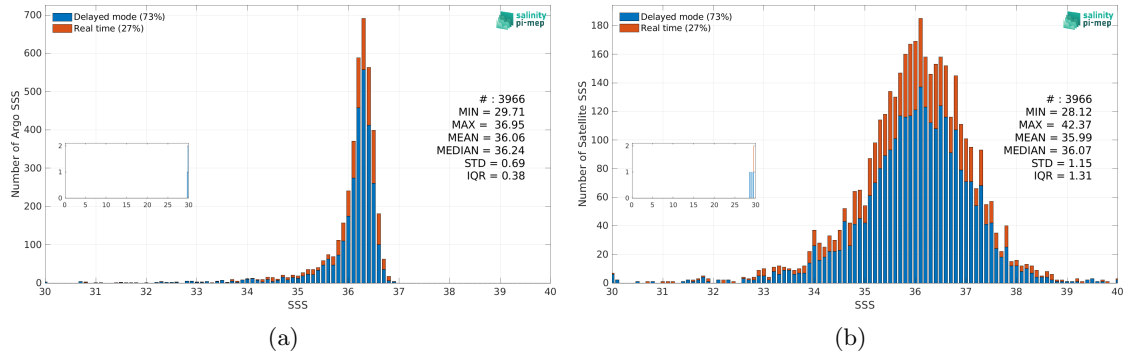
Figure 3: Histograms of SSS from Argo (a) and SMOS SSS L2Q v333 - 0.25 Deg (CATDS-CPDC) (b) considering all match-up pairs per bins of 0.1 over the Gulf of Mexico Pi-MEP region and for the full satellite product period.
