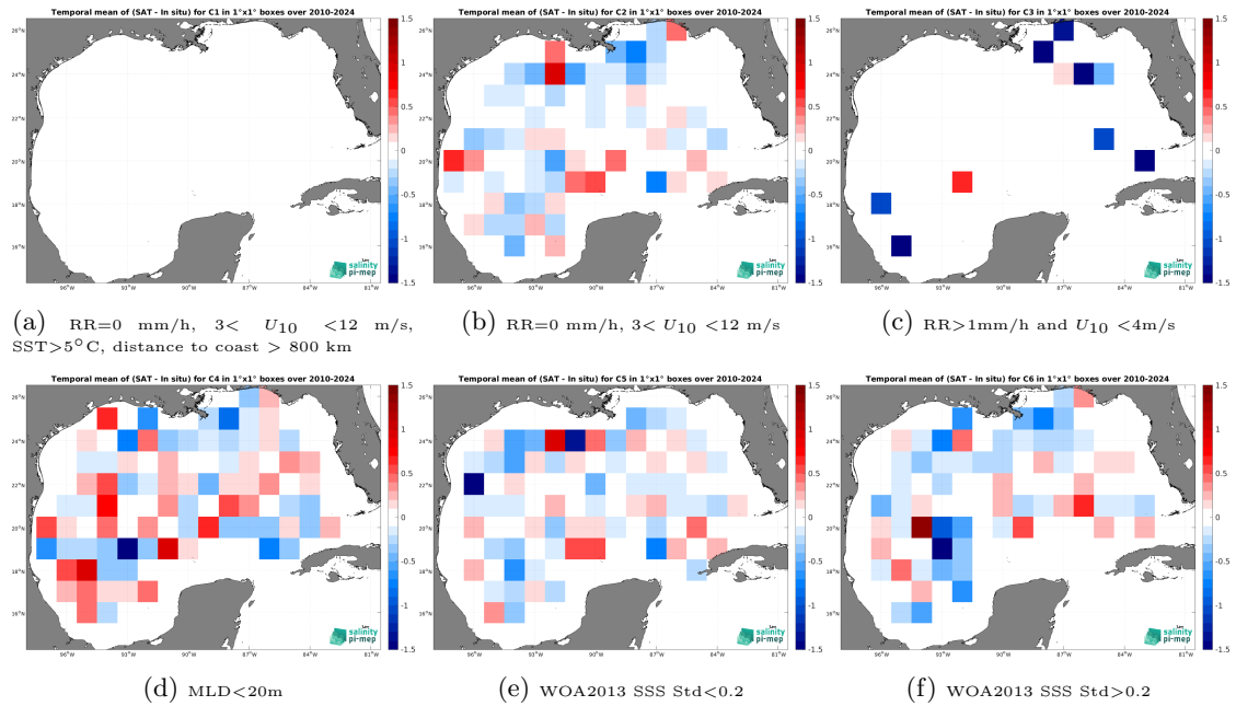
Figure 14: Temporal mean gridded over spatial boxes of size 1^\circ \times 1^\circ of \Delta\text{SSS} (SMOS SSS L2Q v333 - 0.25 Deg (CATDS-CPDC) - Argo) for 6 different subdatasets corresponding to:RR=0 mm/h, 3 < U_{10} < 12 m/s, SST > 5°C, distance to coast > 800 km (a), RR=0 mm/h, 3 < U_{10} < 12 m/s (b), RR > 1mm/h and U_{10} < 4 m/s (c),MLD < 20m (d),WOA2013 SSS Std < 0.2 (e),WOA2013 SSS Std > 0.2 (f).
