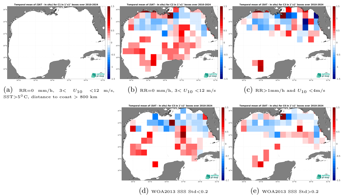
Figure 14: Temporal mean gridded over spatial boxes of size 1^\circ \times 1^\circ of \Delta\text{SSS} (SMOS SSS L3 v332 - 9 Days (CATDS-CPDC) - TSG (SAMOS)) for 5 different subdatasets corresponding to:RR=0 mm/h, 3 < U_{10} < 12 m/s, SST > 5^\circ\text{C} , distance to coast > 800 km (a), RR=0 mm/h, 3 < U_{10} < 12 m/s (b), RR > 1 mm/h and U_{10} < 4 m/s (c), WOA2013 SSS Std < 0.2 (d), WOA2013 SSS Std > 0.2 (e).
