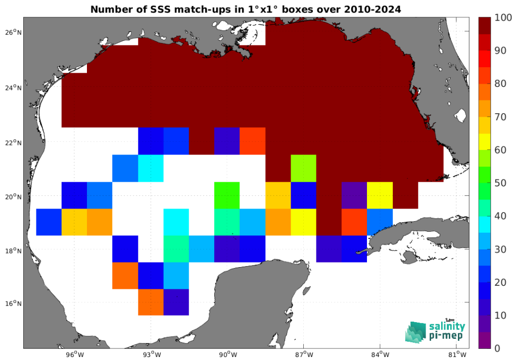
Figure 5: Number of SSS match-ups between TSG (SAMOS) SSS and the SMOS SSS L3 v332 - 9 Days (CATDS-CPDC) SSS product for the Gulf of Mexico Pi-MEP region over 1^\circ \times 1^\circ boxes and for the full satellite product period.
