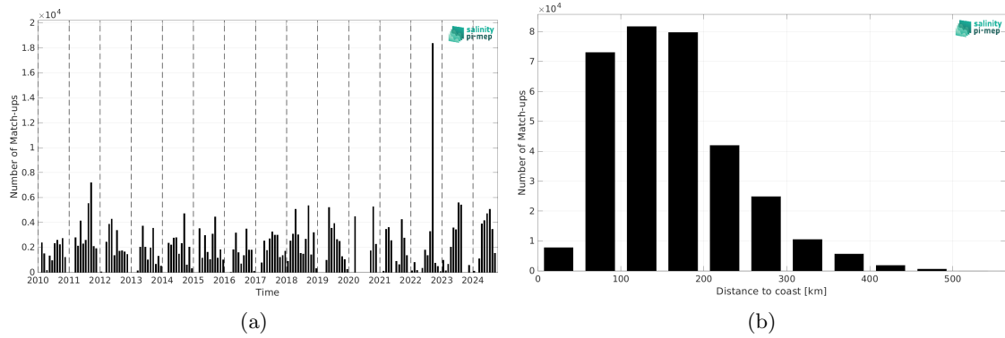
Figure 2: Number of match-ups between TSG (SAMOS) and SMOS SSS L3 v332 - 9 Days (CATDS-CPDC) SSS as a function of time (a) and as function of the distance to coast (b) over the Gulf of Mexico Pi-MEP region and for the full satellite product period.
