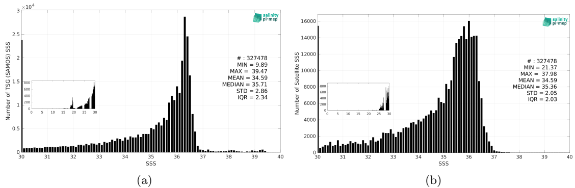
Figure 3: Histograms of SSS from TSG (SAMOS) (a) and SMOS SSS L3 v332 - 9 Days (CATDS-CPDC) (b) considering all match-up pairs per bins of 0.1 over the Gulf of Mexico Pi-MEP region and for the full satellite product period.
