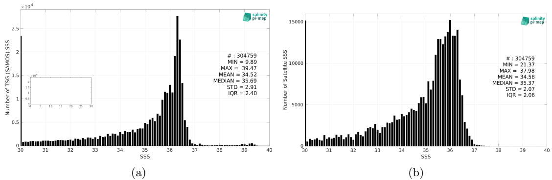
Figure 2: Histograms of SSS from TSG (SAMOS) (a) and SMOS SSS L3 v332 - 9 Days (CATDS-CPDC) (b) considering all match-up pairs per bins of 0.1 over the Gulf of Mexico Pi-MEP region and for the full satellite product period.
