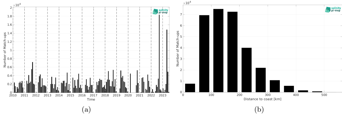
Figure 1: Number of match-ups between TSG (SAMOS) and SMOS SSS L3 v332 - 9 Days (CATDS-CPDC) SSS as a function of time (a) and as function of the distance to coast (b) over the Gulf of Mexico Pi-MEP region and for the full satellite product period.
