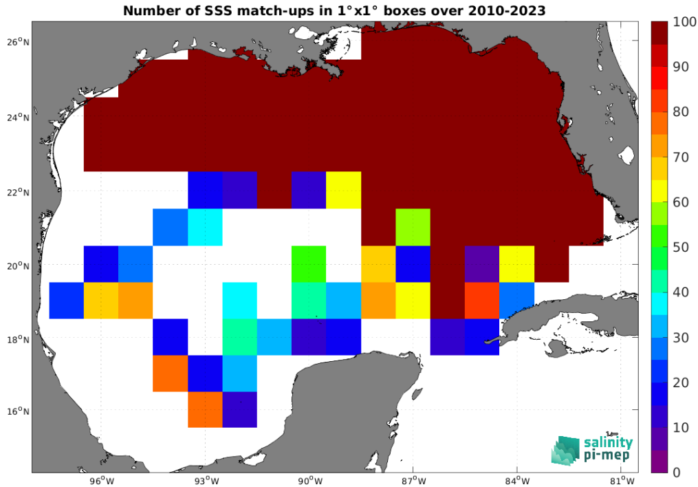
Figure 4: Number of SSS match-ups between TSG (SAMOS) SSS and the SMOS SSS L3 v332 - 9 Days (CATDS-CPDC) SSS product for the Gulf of Mexico Pi-MEP region over 1°x1° boxes and for the full satellite product period.
