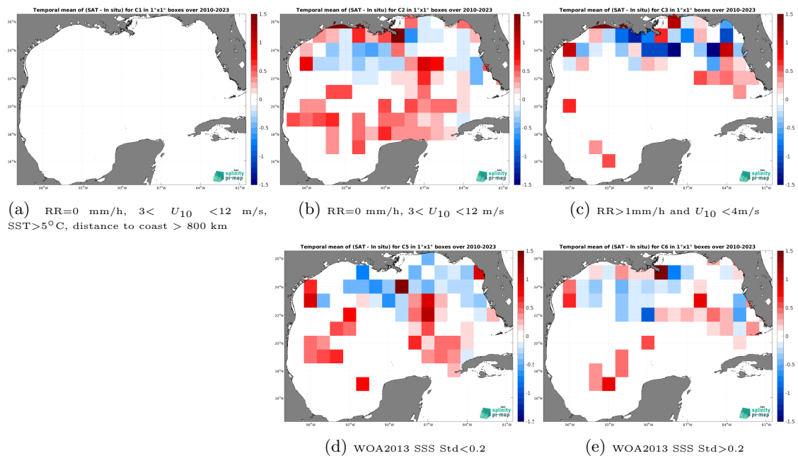
Figure 12: Temporal mean gridded over spatial boxes of size 1^\circ \times 1^\circ of \Delta SSS (SMOS SSS L3 v332 - 9 Days (CATDS-CPDC) - TSG (SAMOS)) for 5 different subdatasets corresponding to:RR=0 mm/h, 3 < U_{10} < 12 m/s, SST >5^\circ C, distance to coast > 800 km (a), RR=0 mm/h, 3 < U_{10} < 12 m/s (b), RR >1 mm/h and U_{10} < 4 m/s (c), WOA2013 SSS Std <0.2 (d), WOA2013 SSS Std >0.2 (e).
