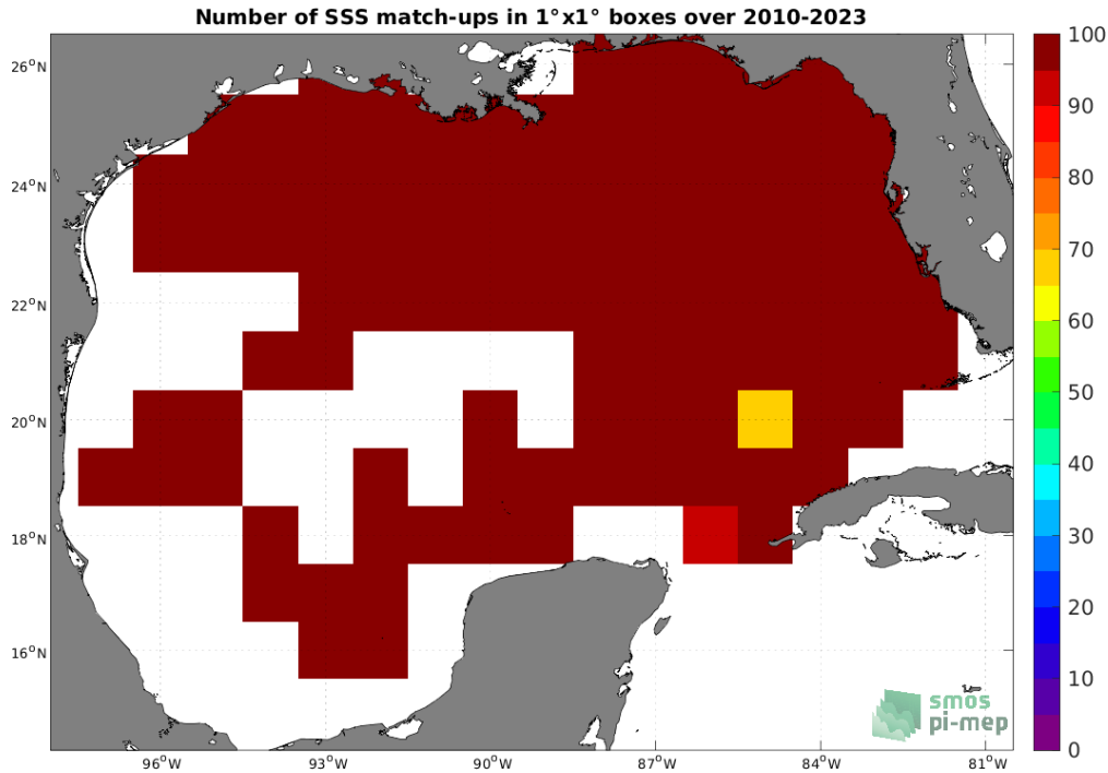
Figure 4: Number of SSS match-ups between TSG (SAMOS) SSS and the SMOS SSS L3 v332 - 9 Days (CATDS-CPDC) SSS product for the Gulf of Mexico Pi-MEP region over 1^\circ \times 1^\circ boxes and for the full satellite product period.
