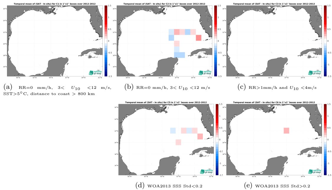
Figure 14: Temporal mean gridded over spatial boxes of size 1^\circ \times 1^\circ of \Delta\text{SSS} (SMOS SSS L3 v332 - 9 Days (CATDS-CPDC) - TSG (GOSUD-Sailing-ship)) for 5 different subdatasets corresponding to:RR=0 mm/h, 3 < U_{10} < 12 m/s, SST>5°C, distance to coast > 800 km (a), RR=0 mm/h, 3 < U_{10} < 12 m/s (b), RR>1mm/h and U_{10} < 4 m/s (c), WOA2013 SSS Std<0.2 (d), WOA2013 SSS Std>0.2 (e).
