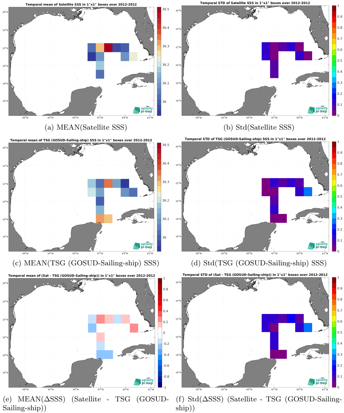
Figure 7: Temporal mean (left) and Std (right) of SSS from SMOS SSS L3 v332 - 9 Days (CATDS-CPDC) (top), TSG (GOSUD-Sailing-ship) (middle), and of \Delta SSS (Satellite - TSG (GOSUD-Sailing-ship)). Only match-up pairs are used to generate these maps.
