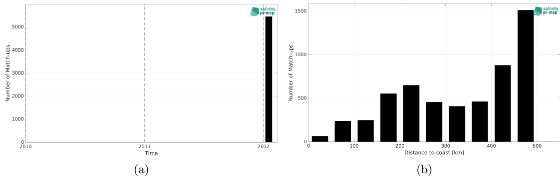
Figure 2: Number of match-ups between TSG (GOSUD-Sailing-ship) and SMOS SSS L3 v332 - 9 Days (CATDS-CPDC) SSS as a function of time (a) and as function of the distance to coast (b) over the Gulf of Mexico Pi-MEP region and for the full satellite product period.
