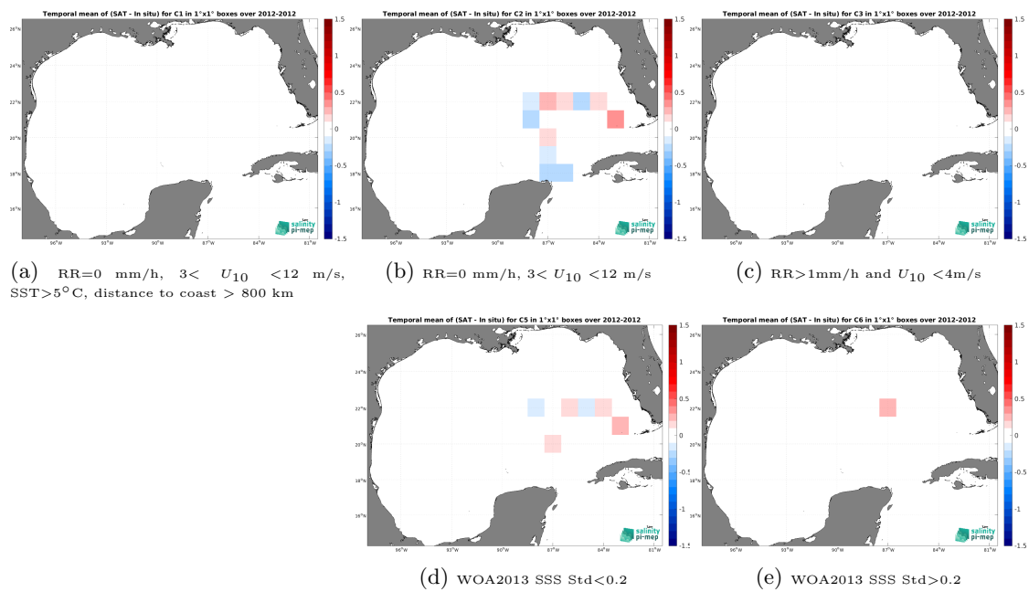
Figure 14: Temporal mean gridded over spatial boxes of size 1^\circ \times 1^\circ of \Delta SSS (SMOS SSS L3 v332 - 9 Days (CATDS-CPDC) - TSG (GOSUD-Sailing-ship)) for 5 different subdatasets corresponding to:RR=0 mm/h, 3 < U_{10} < 12 m/s, SST >5^\circ C, distance to coast > 800 km (a), RR=0 mm/h, 3 < U_{10} < 12 m/s (b), RR >1 mm/h and U_{10} < 4 m/s (c), WOA2013 SSS Std <0.2 (d), WOA2013 SSS Std >0.2 (e).
