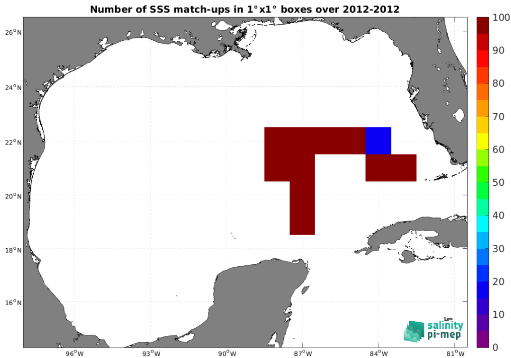
Figure 5: Number of SSS match-ups between TSG (GOSUD-Sailing-ship) SSS and the SMOS SSS L3 v332 - 9 Days (CATDS-CPDC) SSS product for the Gulf of Mexico Pi-MEP region over 1^\circ \times 1^\circ boxes and for the full satellite product period.
