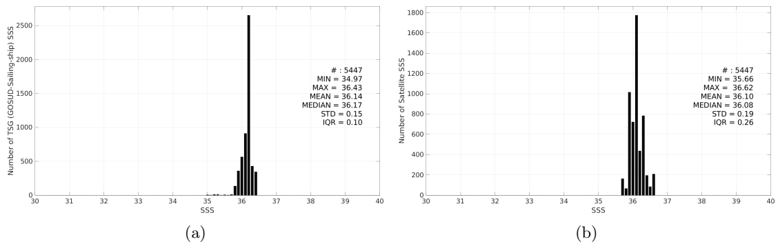
Figure 3: Histograms of SSS from TSG (GOSUD-Sailing-ship) (a) and SMOS SSS L3 v332 - 9 Days (CATDS-CPDC) (b) considering all match-up pairs per bins of 0.1 over the Gulf of Mexico Pi-MEP region and for the full satellite product period.
