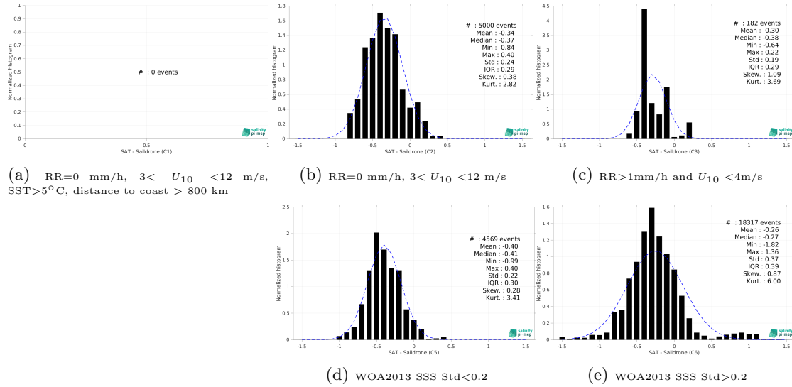
Figure 15: Normalized histogram of \Delta SSS (SMOS SSS L3 v332 - 9 Days (CATDS-CPDC) - Saldrone) for 5 different subdatasets corresponding to: RR=0 mm/h, 3 < U_{10} < 12 m/s, SST > 5°C, distance to coast > 800 km (a), RR=0 mm/h, 3 < U_{10} < 12 m/s (b), RR > 1mm/h and U_{10} < 4 m/s (c), WOA2013 SSS Std < 0.2 (d), WOA2013 SSS Std > 0.2 (e).
