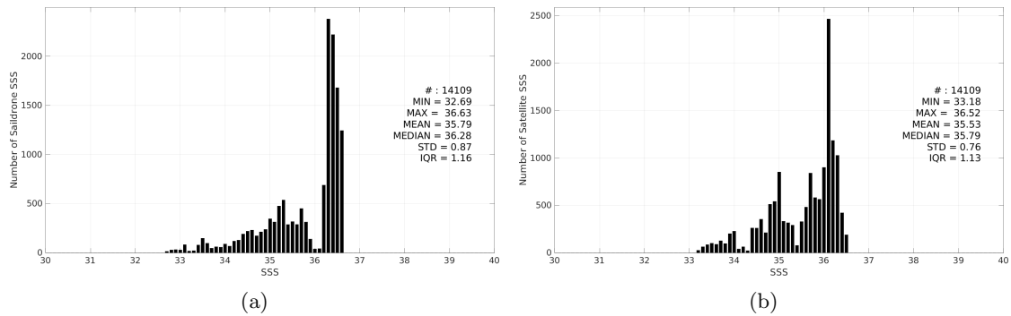
Figure 3: Histograms of SSS from Saildrone (a) and SMOS SSS L3 v332 - 9 Days (CATDS-CPDC) (b) considering all match-up pairs per bins of 0.1 over the Gulf of Mexico Pi-MEP region and for the full satellite product period.
