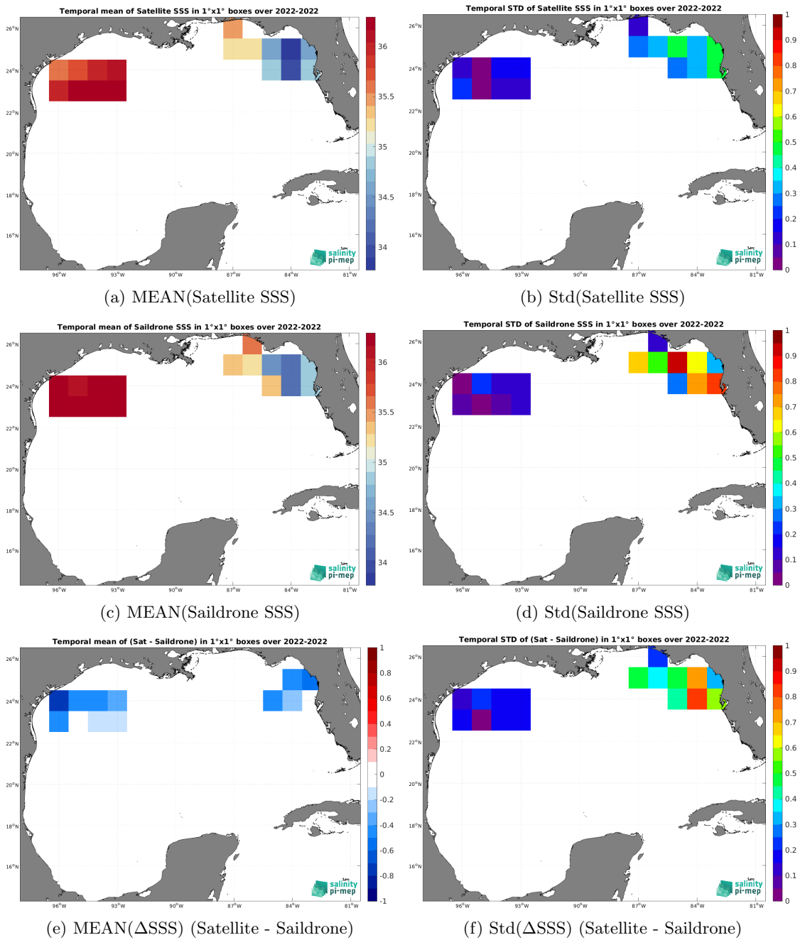
Figure 7: Temporal mean (left) and Std (right) of SSS from SMOS SSS L3 v332 - 9 Days (CATDS-CPDC) (top), Saildrone (middle), and of \Delta SSS (Satellite - Saildrone). Only match-up pairs are used to generate these maps.
