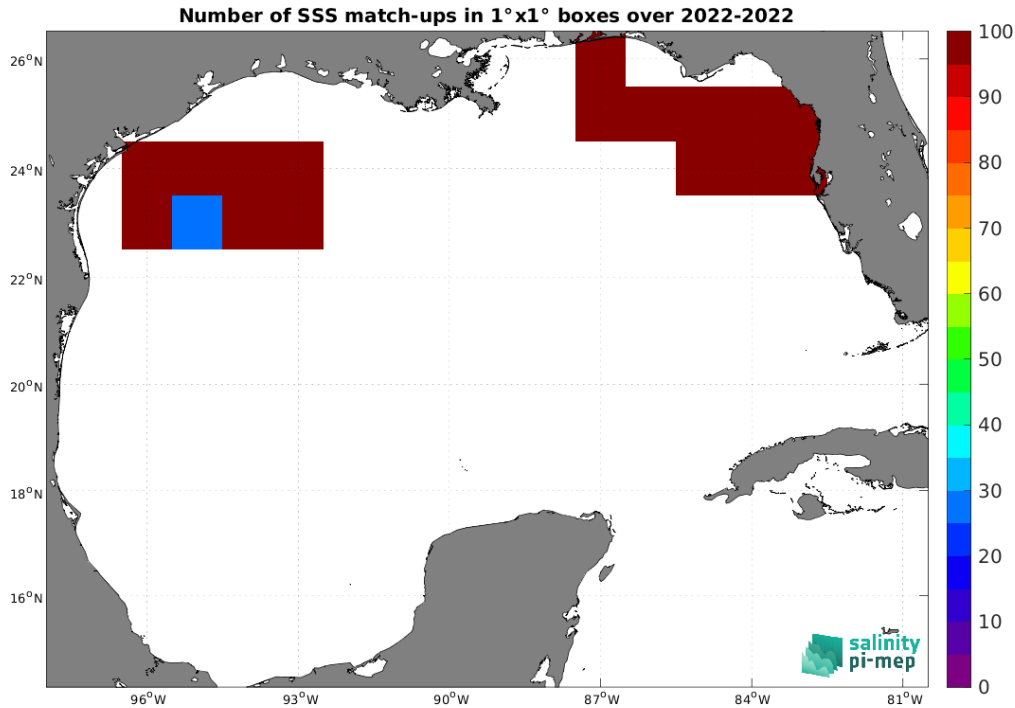
Figure 5: Number of SSS match-ups between Saildrone SSS and the SMOS SSS L3 v332 - 9 Days (CATDS-CPDC) SSS product for the Gulf of Mexico Pi-MEP region over 1^\circ \times 1^\circ boxes and for the full satellite product period.
