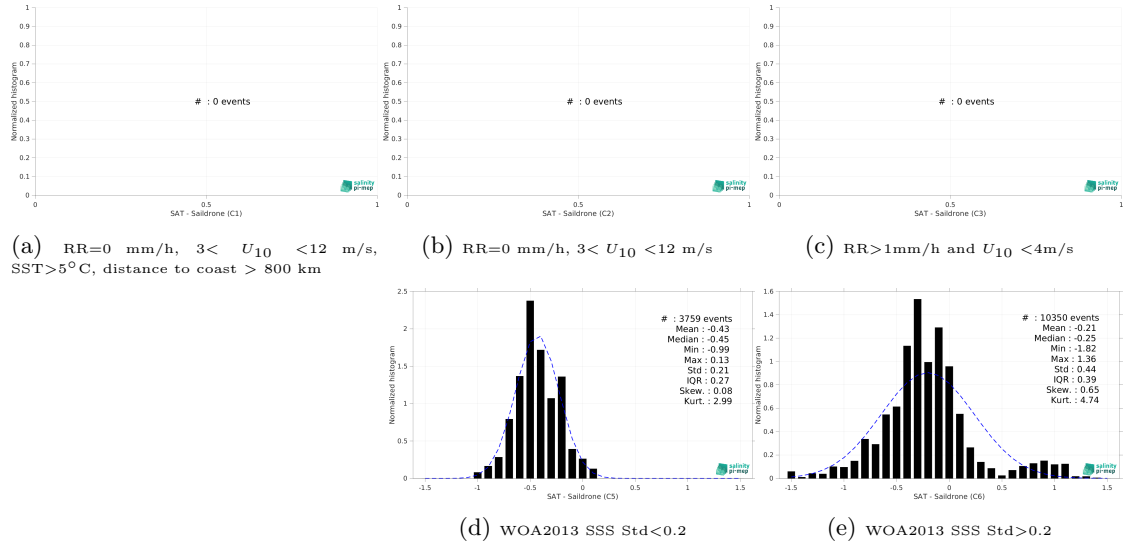
Figure 15: Normalized histogram of \Delta SSS (SMOS SSS L3 v332 - 9 Days (CATDS-CPDC) - Saildrone) for 5 different subdatasets corresponding to: RR=0 mm/h, 3 < U_{10} < 12 m/s, SST>5°C, distance to coast > 800 km (a), RR=0 mm/h, 3 < U_{10} < 12 m/s (b), RR>1mm/h and U_{10} < 4 m/s (c), WOA2013 SSS Std<0.2 (d), WOA2013 SSS Std>0.2 (e).
