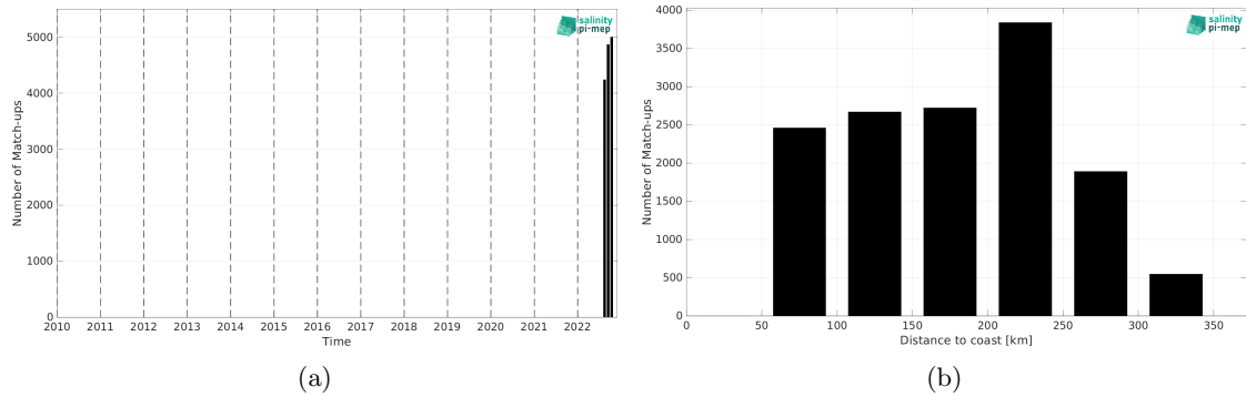
Figure 2: Number of match-ups between Saildrone and SMOS SSS L3 v332 - 9 Days (CATDS-CPDC) SSS as a function of time (a) and as function of the distance to coast (b) over the Gulf of Mexico Pi-MEP region and for the full satellite product period.
