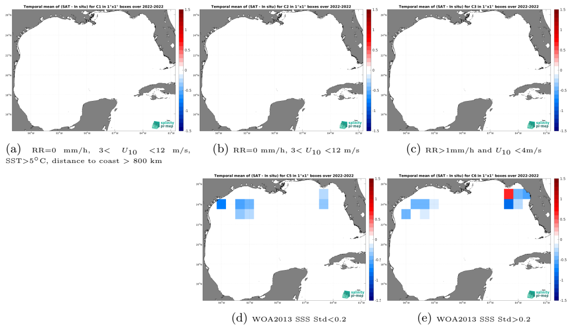
Figure 14: Temporal mean gridded over spatial boxes of size 1^\circ \times 1^\circ of \Delta SSS (SMOS SSS L3 v332 - 9 Days (CATDS-CPDC) - Sairdrone) for 5 different subdatasets corresponding to:RR=0 mm/h, 3 < U_{10} < 12 m/s, SST > 5°C, distance to coast > 800 km (a), RR=0 mm/h, 3 < U_{10} < 12 m/s (b), RR > 1mm/h and U_{10} < 4 m/s (c), WOA2013 SSS Std < 0.2 (d), WOA2013 SSS Std > 0.2 (e).
