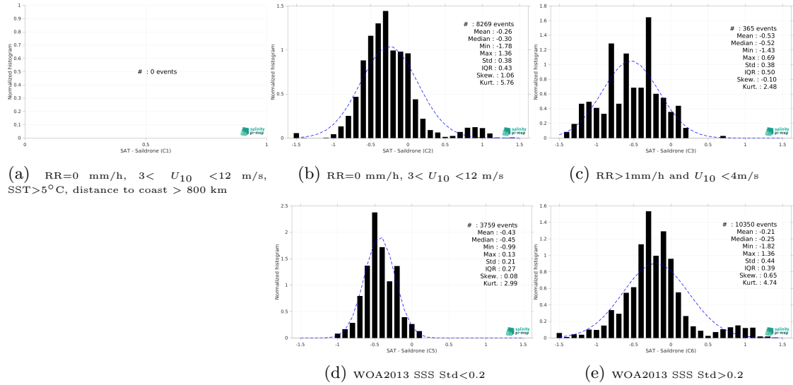
Figure 13: Normalized histogram of \Delta SSS (SMOS SSS L3 v332 - 9 Days (CATDS-CPDC) - Saldrone) for 5 different subdatasets corresponding to: RR=0 mm/h, 3 < U_{10} < 12 m/s, SST > 5°C, distance to coast > 800 km (a), RR=0 mm/h, 3 < U_{10} < 12 m/s (b), RR > 1mm/h and U_{10} < 4 m/s (c), WOA2013 SSS Std < 0.2 (d), WOA2013 SSS Std > 0.2 (e).
