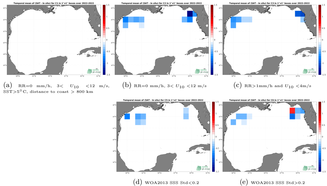
Figure 12: Temporal mean gridded over spatial boxes of size 1^{\circ}\times 1^{\circ} of \Delta\text{SSS} (SMOS SSS L3 v332 - 9 Days (CATDS-CPDC) - Saildrone) for 5 different subdatasets corresponding to:RR=0 mm/h, 3 < U_{10} < 12 m/s, SST >5^{\circ}\text{C} , distance to coast > 800 km (a), RR=0 mm/h, 3 < U_{10} < 12 m/s (b), RR >1 mm/h and U_{10} < 4 m/s (c), WOA2013 SSS Std <0.2 (d), WOA2013 SSS Std >0.2 (e).
