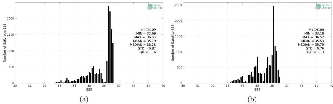
Figure 2: Histograms of SSS from Saildrone (a) and SMOS SSS L3 v332 - 9 Days (CATDS-CPDC) (b) considering all match-up pairs per bins of 0.1 over the Gulf of Mexico Pi-MEP region and for the full satellite product period.
