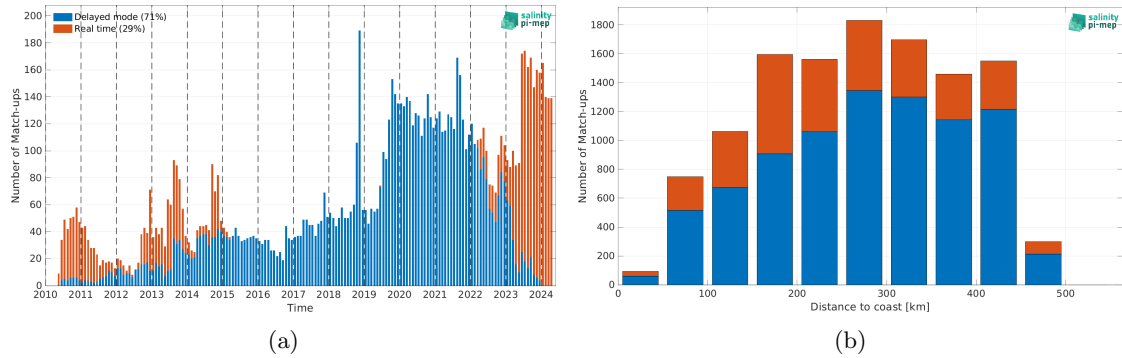
Figure 2: Number of match-ups between Argo and SMOS SSS L3 v332 - 9 Days (CATDS-CPDC) SSS as a function of time (a) and as function of the distance to coast (b) over the Gulf of Mexico Pi-MEP region and for the full satellite product period.
