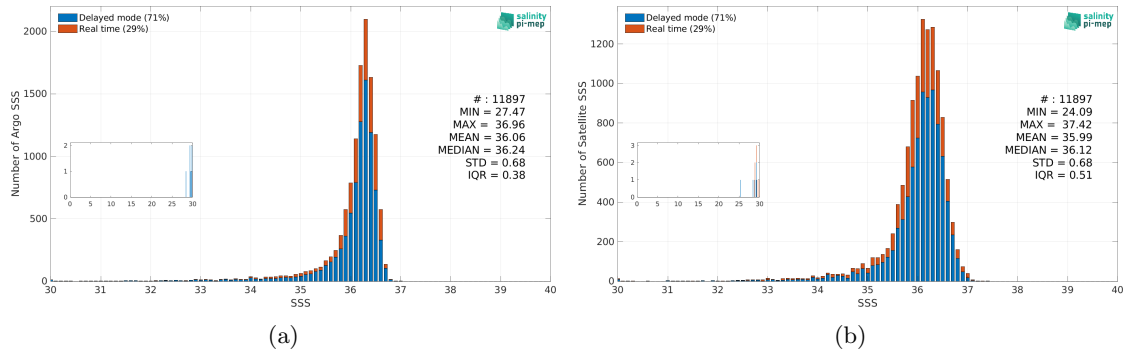
Figure 3: Histograms of SSS from Argo (a) and SMOS SSS L3 v332 - 9 Days (CATDS-CPDC) (b) considering all match-up pairs per bins of 0.1 over the Gulf of Mexico Pi-MEP region and for the full satellite product period.
