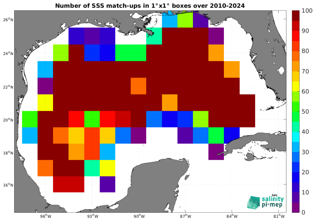
Figure 5: Number of SSS match-ups between Argo SSS and the SMOS SSS L3 v332 - 9 Days (CATDS-CPDC) SSS product for the Gulf of Mexico Pi-MEP region over 1^\circ \times 1^\circ boxes and for the full satellite product period.
