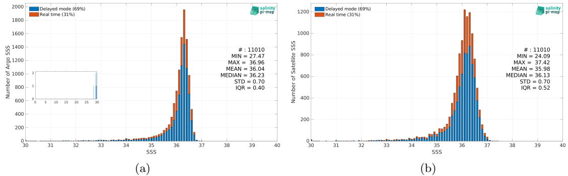
Figure 2: Histograms of SSS from Argo (a) and SMOS SSS L3 v332 - 9 Days (CATDS-CPDC) (b) considering all match-up pairs per bins of 0.1 over the Gulf of Mexico Pi-MEP region and for the full satellite product period.
