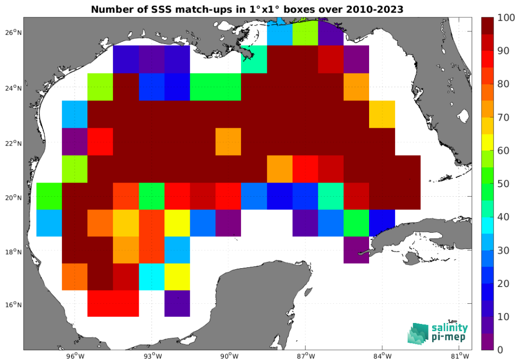
Figure 4: Number of SSS match-ups between Argo SSS and the SMOS SSS L3 v332 - 9 Days (CATDS-CPDC) SSS product for the Gulf of Mexico Pi-MEP region over 1^\circ \times 1^\circ boxes and for the full satellite product period.
