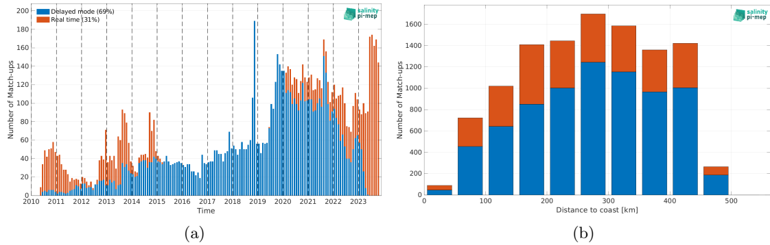
Figure 1: Number of match-ups between Argo and SMOS SSS L3 v332 - 9 Days (CATDS-CPDC) SSS as a function of time (a) and as function of the distance to coast (b) over the Gulf of Mexico Pi-MEP region and for the full satellite product period.
