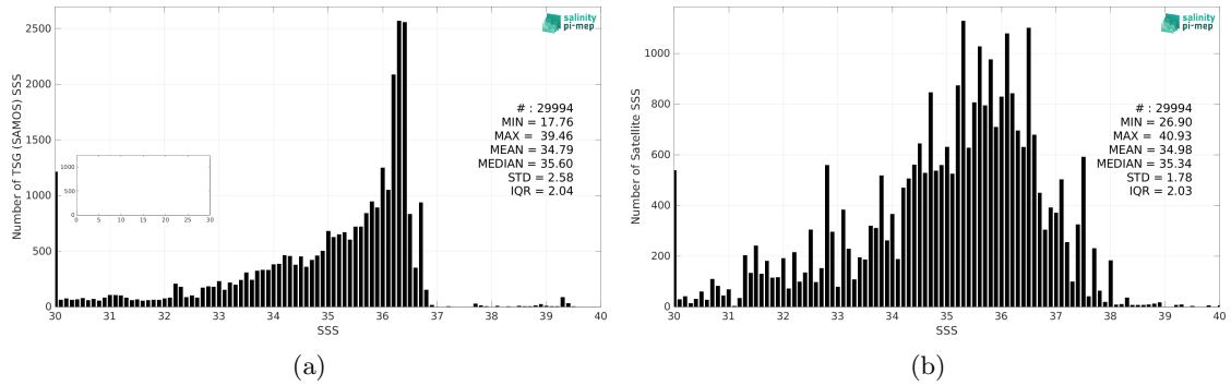
Figure 2: Histograms of SSS from TSG (SAMOS) (a) and SMOS SSS L2Q v331 - 0.25 Deg (CATDS-CPDC) (b) considering all match-up pairs per bins of 0.1 over the Gulf of Mexico Pi-MEP region and for the full satellite product period.
