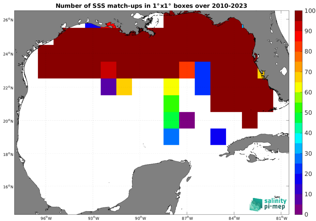
Figure 4: Number of SSS match-ups between TSG (SAMOS) SSS and the SMOS SSS L2Q v331 - 0.25 Deg (CATDS-CPDC) SSS product for the Gulf of Mexico Pi-MEP region over 1^\circ \times 1^\circ boxes and for the full satellite product period.
