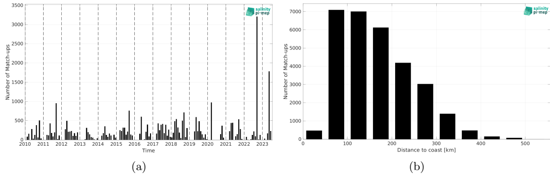
Figure 1: Number of match-ups between TSG (SAMOS) and SMOS SSS L2Q v331 - 0.25 Deg (CATDS-CPDC) SSS as a function of time (a) and as function of the distance to coast (b) over the Gulf of Mexico Pi-MEP region and for the full satellite product period.
