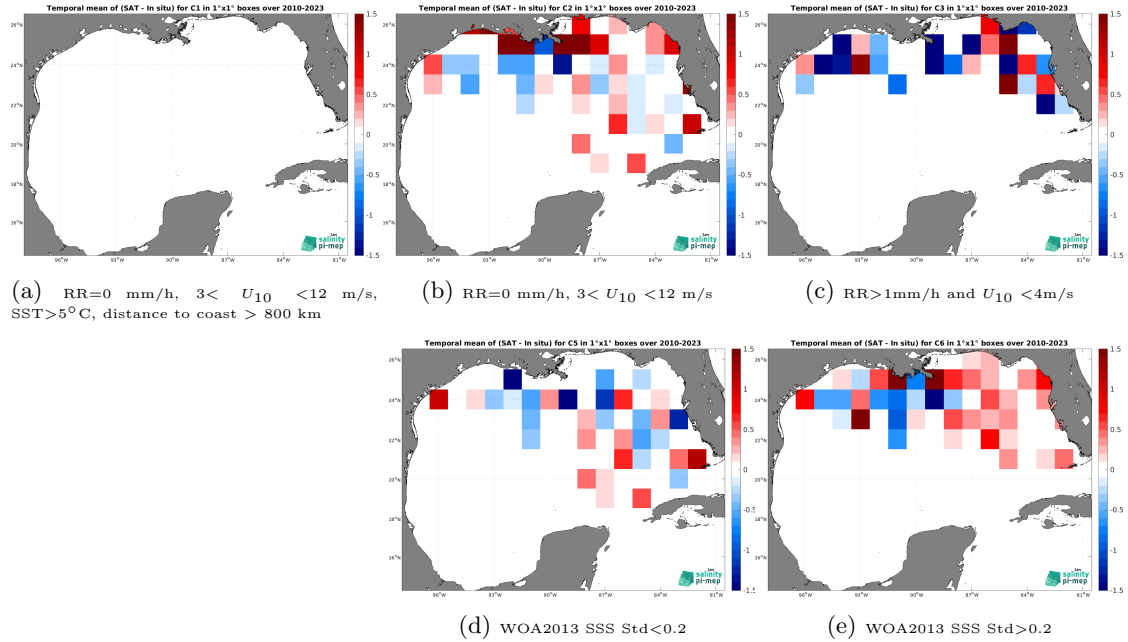
Figure 12: Temporal mean gridded over spatial boxes of size 1^{\circ}\times 1^{\circ} of \Delta\text{SSS} (SMOS SSS L2Q v331 - 0.25 Deg (CATDS-CPDC) - TSG (SAMOS)) for 5 different subdatasets corresponding to:RR=0 mm/h, 3 < U_{10} < 12 m/s, SST >5^{\circ}\text{C} , distance to coast > 800 km (a), RR=0 mm/h, 3 < U_{10} < 12 m/s (b), RR >1 mm/h and U_{10} < 4 m/s (c), WOA2013 SSS Std <0.2 (d), WOA2013 SSS Std >0.2 (e).
