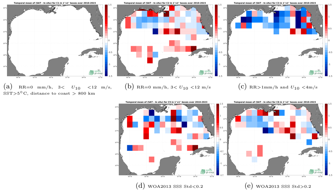
Figure 12: Temporal mean gridded over spatial boxes of size 1^\circ \times 1^\circ of \Delta SSS (SMOS SSS L2Q v331 - 0.25 Deg (CATDS-CPDC) - TSG (SAMOS)) for 5 different subdatasets corresponding to:RR=0 mm/h, 3 < U_{10} < 12 m/s, SST >5^\circ C, distance to coast > 800 km (a), RR=0 mm/h, 3 < U_{10} < 12 m/s (b), RR >1 mm/h and U_{10} < 4 m/s (c), WOA2013 SSS Std <0.2 (d), WOA2013 SSS Std >0.2 (e).
