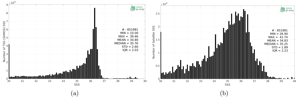
Figure 2: Histograms of SSS from TSG (SAMOS) (a) and SMOS SSS L2Q v331 - 0.25 Deg (CATDS-CPDC) (b) considering all match-up pairs per bins of 0.1 over the Gulf of Mexico Pi-MEP region and for the full satellite product period.
