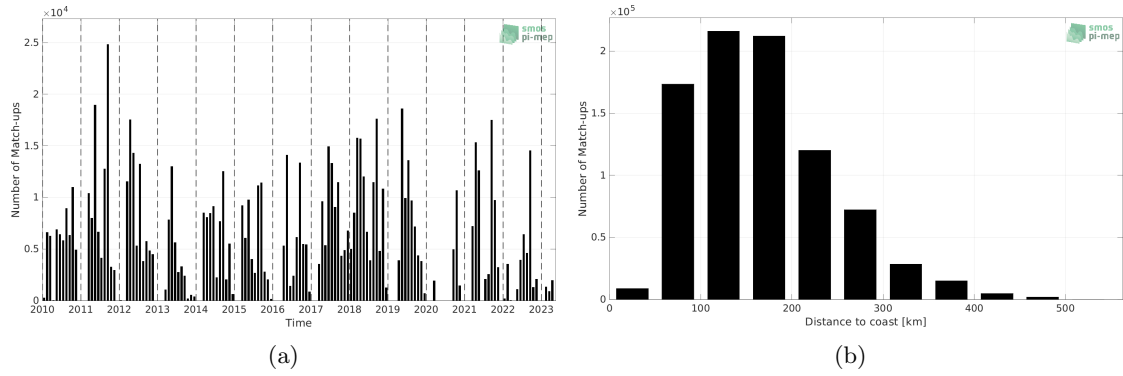
Figure 1: Number of match-ups between TSG (SAMOS) and SMOS SSS L2Q v331 - 0.25 Deg (CATDS-CPDC) SSS as a function of time (a) and as function of the distance to coast (b) over the Gulf of Mexico Pi-MEP region and for the full satellite product period.
