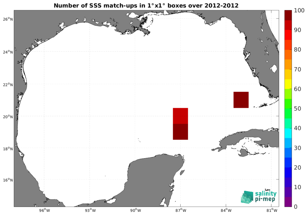
Figure 4: Number of SSS match-ups between TSG (GOSUD-Sailing-ship) SSS and the SMOS SSS L2Q v331 - 0.25 Deg (CATDS-CPDC) SSS product for the Gulf of Mexico Pi-MEP region over 1^\circ \times 1^\circ boxes and for the full satellite product period.
