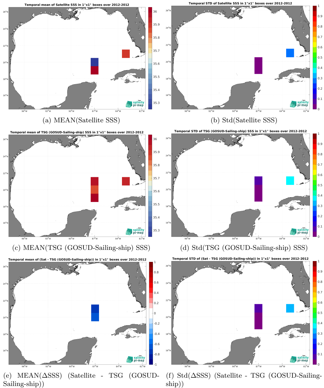
Figure 6: Temporal mean (left) and Std (right) of SSS from SMOS SSS L2Q v331 - 0.25 Deg (CATDS-CPDC) (top), TSG (GOSUD-Sailing-ship) (middle), and of \Delta SSS (Satellite - TSG (GOSUD-Sailing-ship)). Only match-up pairs are used to generate these maps.
