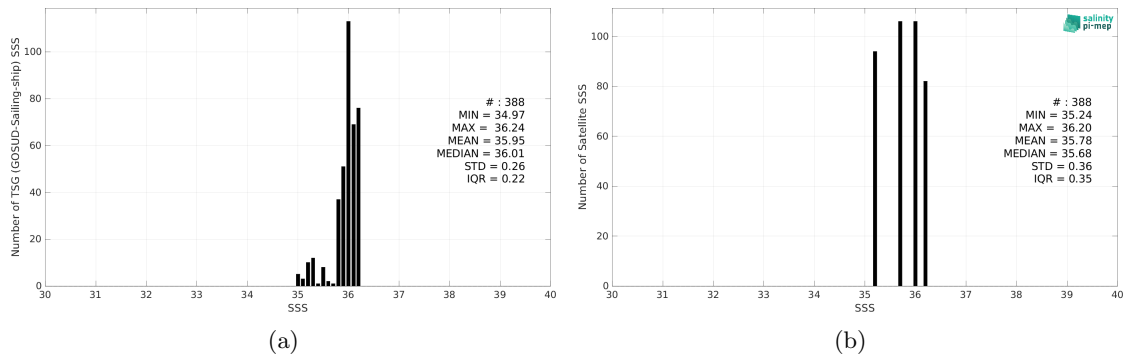
Figure 2: Histograms of SSS from TSG (GOSUD-Sailing-ship) (a) and SMOS SSS L2Q v331 - 0.25 Deg (CATDS-CPDC) (b) considering all match-up pairs per bins of 0.1 over the Gulf of Mexico Pi-MEP region and for the full satellite product period.
