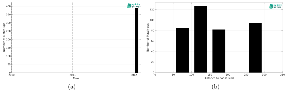
Figure 1: Number of match-ups between TSG (GOSUD-Sailing-ship) and SMOS SSS L2Q v331 - 0.25 Deg (CATDS-CPDC) SSS as a function of time (a) and as function of the distance to coast (b) over the Gulf of Mexico Pi-MEP region and for the full satellite product period.
