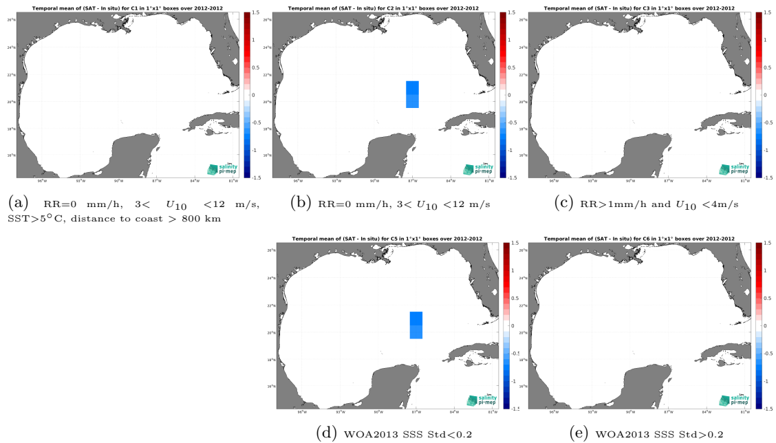
Figure 12: Temporal mean gridded over spatial boxes of size 1^{\circ}\times 1^{\circ} of \Delta SSS (SMOS SSS L2Q v331 - 0.25 Deg (CATDS-CPDC) - TSG (GOSUD-Sailing-ship)) for 5 different subdatasets corresponding to:RR=0 mm/h, 3 < U_{10} < 12 m/s, SST >5^{\circ}\text{C} , distance to coast > 800 km (a), RR=0 mm/h, 3 < U_{10} < 12 m/s (b), RR >1 mm/h and U_{10} < 4 m/s (c), WOA2013 SSS Std <0.2 (d), WOA2013 SSS Std >0.2 (e).
