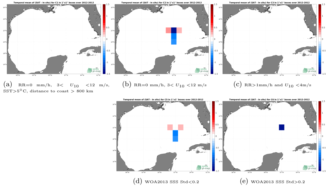
Figure 12: Temporal mean gridded over spatial boxes of size 1^\circ \times 1^\circ of \Delta SSS (SMOS SSS L2Q v331 - 0.25 Deg (CATDS-CPDC) - TSG (GOSUD-Sailing-ship)) for 5 different subdatasets corresponding to:RR=0 mm/h, 3 < U_{10} < 12 m/s, SST >5^\circ\text{C} , distance to coast > 800 km (a), RR=0 mm/h, 3 < U_{10} < 12 m/s (b), RR >1 mm/h and U_{10} < 4 m/s (c), WOA2013 SSS Std <0.2 (d), WOA2013 SSS Std >0.2 (e).
