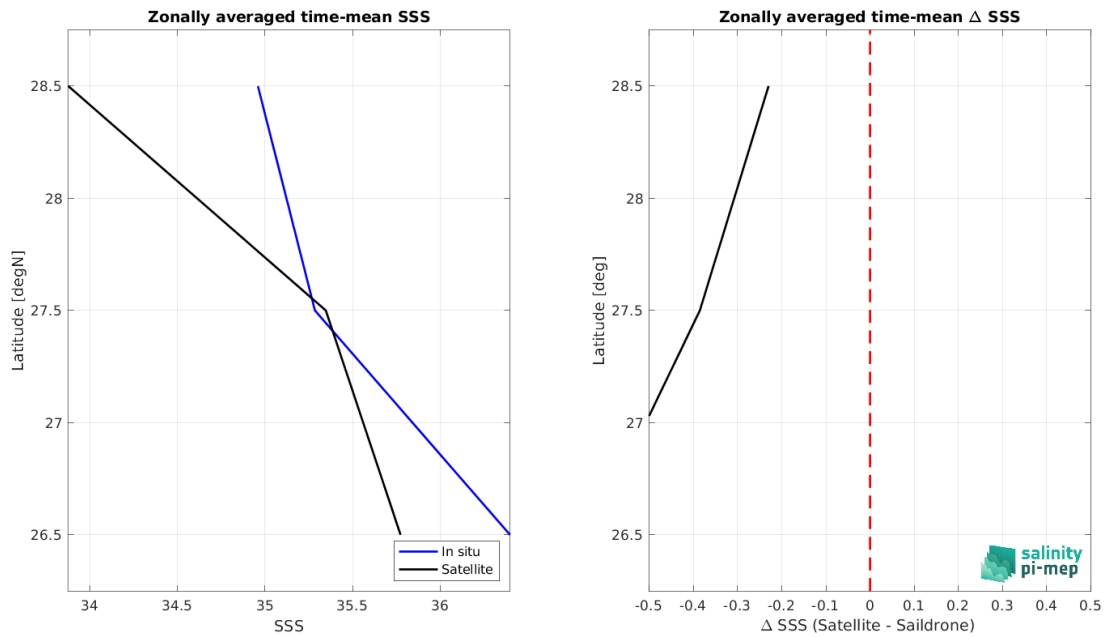
Figure 8: Left panel: Zonal mean SSS from SMOS SSS L2Q v331 - 0.25 Deg (CATDS-CPDC) satellite product (black) and from Sairdron (blue). Right panel: Zonal mean of \Delta SSS (Satellite - Sairdron) for all the collected Pi-MEP match-up pairs estimated over the full satellite product period.
