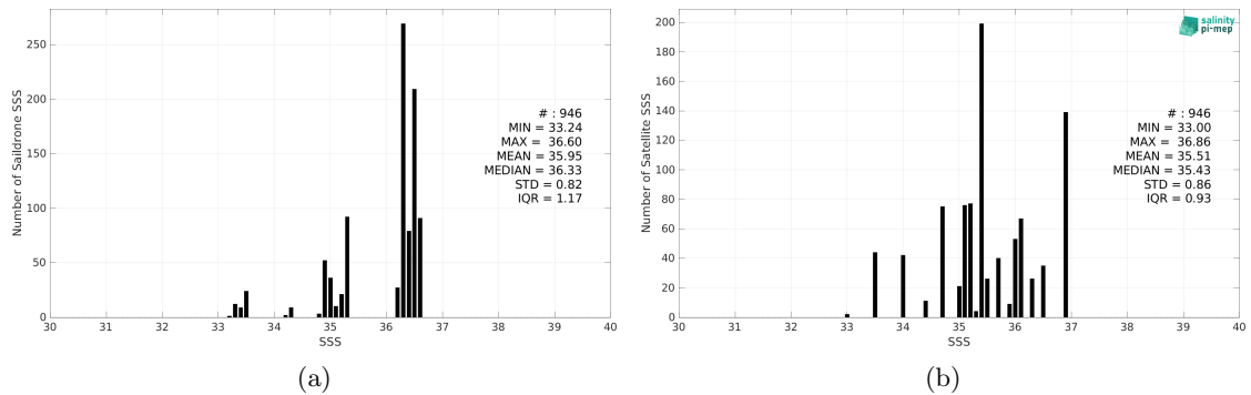
Figure 2: Histograms of SSS from Saildrone (a) and SMOS SSS L2Q v331 - 0.25 Deg (CATDS-CPDC) (b) considering all match-up pairs per bins of 0.1 over the Gulf of Mexico Pi-MEP region and for the full satellite product period.
