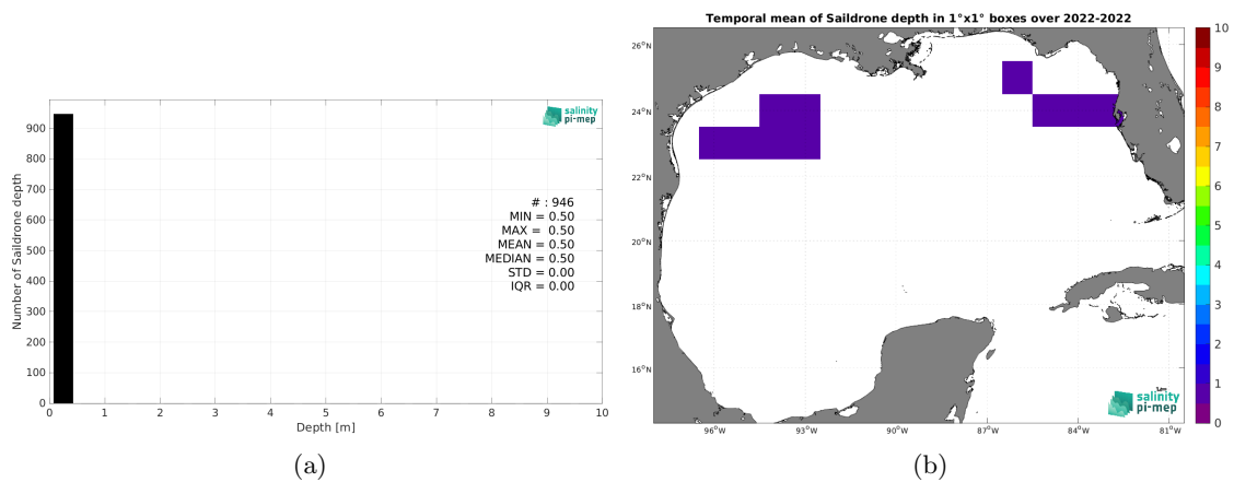
Figure 3: Histograms of the depth of the upper level SSS measurements from Sairdron in the Match-up DataBase for the Gulf of Mexico Pi-MEP region (a) and temporal mean spatial distribution of pressure of the in situ SSS data over 1^\circ \times 1^\circ boxes and for the full satellite product period (b).
