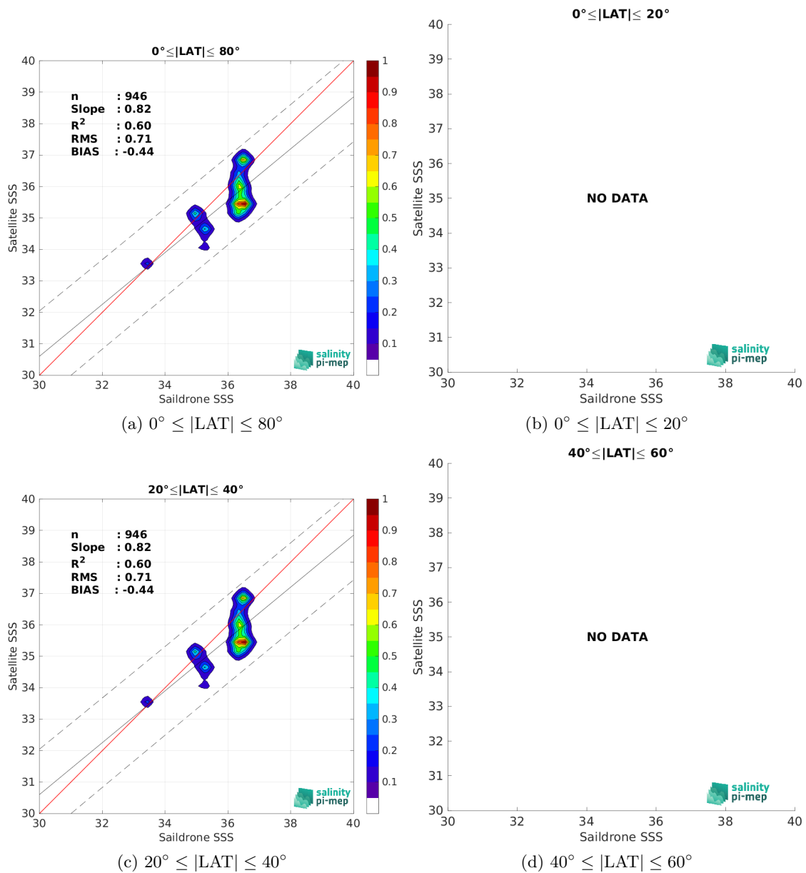
Figure 9: Contour maps of the concentration of SMOS SSS L2Q v331 - 0.25 Deg (CATDS-CPDC) SSS (y-axis) versus Saildrone SSS (x-axis) at match-up pairs for different latitude bands. For each plot, the red line shows x=y . The black thin and dashed lines indicate a linear fit through the data cloud and the \pm 95\% confidence levels, respectively. The number match-up pairs n , the slope and R^2 coefficient of the linear fit, the root mean square (RMS) and the mean bias between satellite and in situ data are indicated for each latitude band in each plots.
