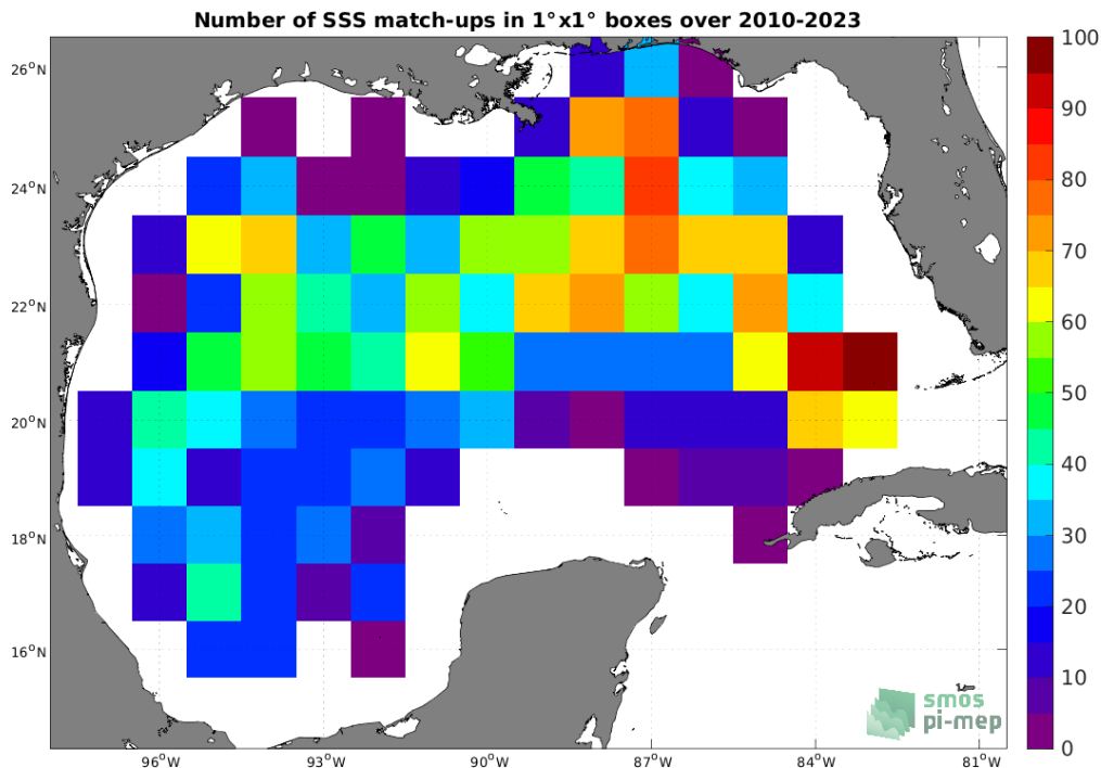
Figure 4: Number of SSS match-ups between Argo SSS and the SMOS SSS L2Q v331 - 0.25 Deg (CATDS-CPDC) SSS product for the Gulf of Mexico Pi-MEP region over 1^\circ \times 1^\circ boxes and for the full satellite product period.
