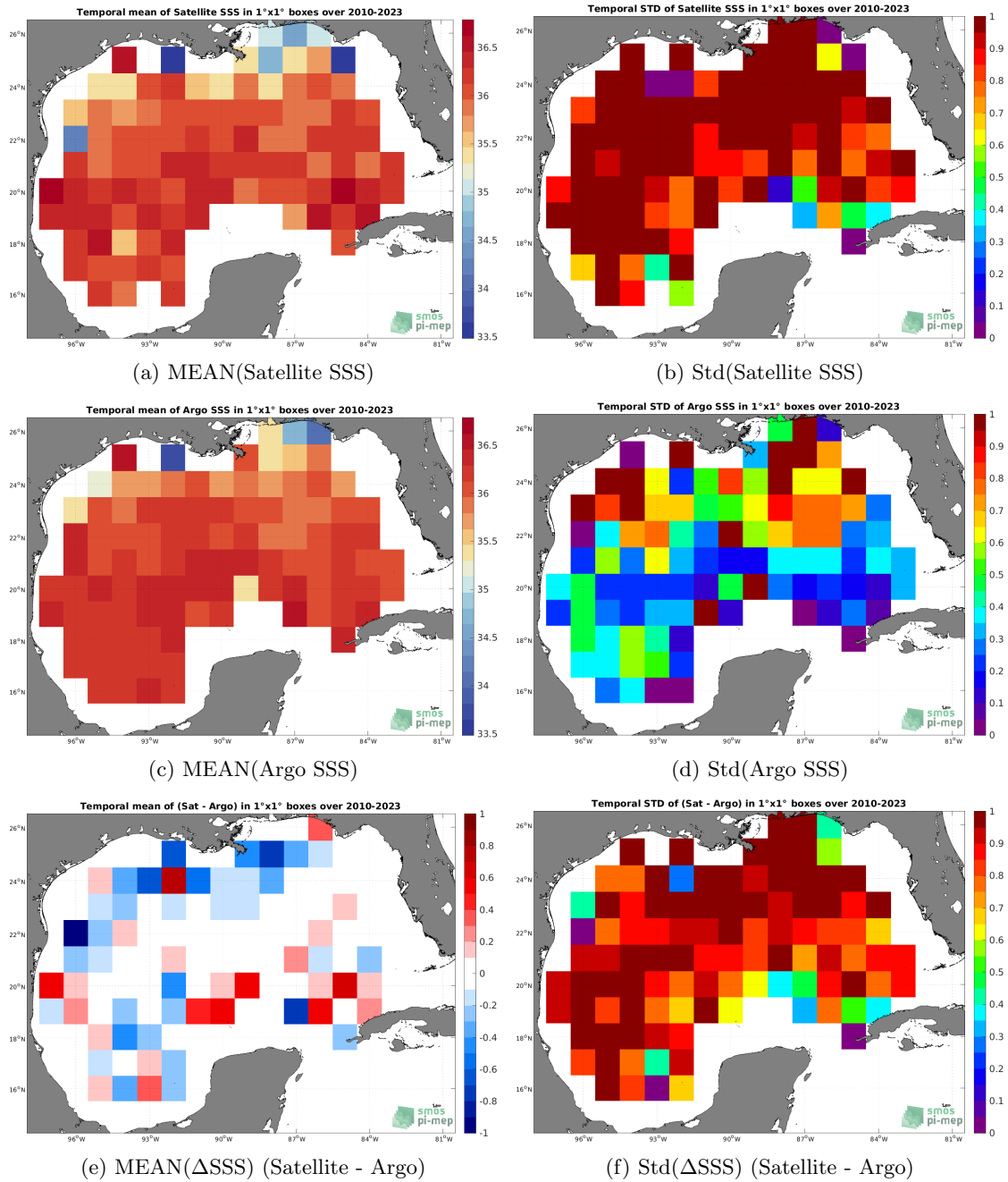
Figure 6: Temporal mean (left) and Std (right) of SSS from SMOS SSS L2Q v331 - 0.25 Deg (CATDS-CPDC) (top), Argo (middle), and of \Delta SSS (Satellite - Argo). Only match-up pairs are used to generate these maps.
