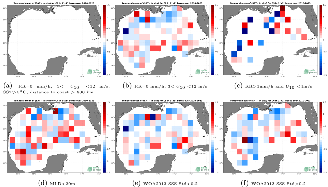
Figure 12: Temporal mean gridded over spatial boxes of size 1^\circ \times 1^\circ of \Delta SSS (SMOS SSS L2Q v331 - 0.25 Deg (CATDS-CPDC) - Argo) for 6 different subdatasets corresponding to:RR=0 mm/h, 3 < U_{10} < 12 m/s, SST > 5^\circ\text{C} , distance to coast > 800 km (a), RR=0 mm/h, 3 < U_{10} < 12 m/s (b), RR > 1 mm/h and U_{10} < 4 m/s (c),MLD < 20 m (d),WOA2013 SSS Std < 0.2 (e),WOA2013 SSS Std > 0.2 (f).
