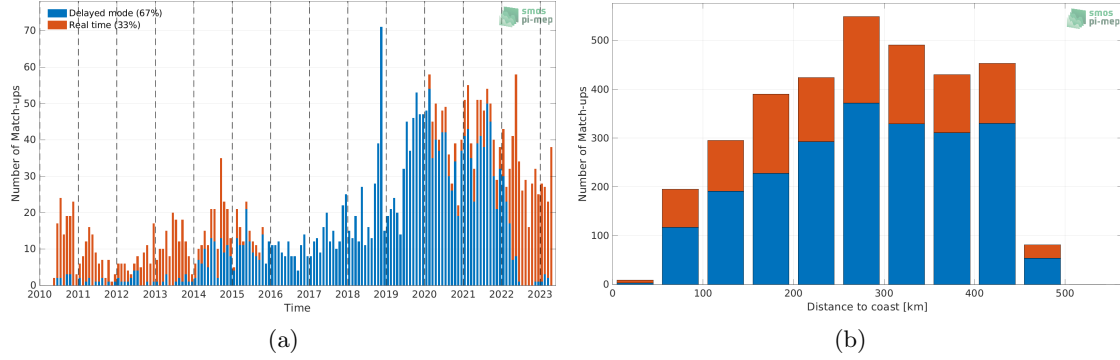
Figure 1: Number of match-ups between Argo and SMOS SSS L2Q v331 - 0.25 Deg (CATDS-CPDC) SSS as a function of time (a) and as function of the distance to coast (b) over the Gulf of Mexico Pi-MEP region and for the full satellite product period.
