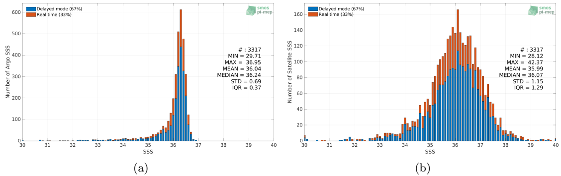
Figure 2: Histograms of SSS from Argo (a) and SMOS SSS L2Q v331 - 0.25 Deg (CATDS-CPDC) (b) considering all match-up pairs per bins of 0.1 over the Gulf of Mexico Pi-MEP region and for the full satellite product period.
