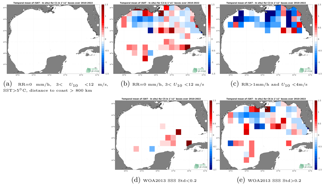
Figure 12: Temporal mean gridded over spatial boxes of size 1^\circ \times 1^\circ of \Delta SSS (SMOS SSS L2Q v330 - 0.25 Deg (CATDS-CPDC) - TSG (SAMOS)) for 5 different subdatasets corresponding to:RR=0 mm/h, 3 < U_{10} < 12 m/s, SST >5^\circ C, distance to coast > 800 km (a), RR=0 mm/h, 3 < U_{10} < 12 m/s (b), RR >1 mm/h and U_{10} < 4 m/s (c), WOA2013 SSS Std <0.2 (d), WOA2013 SSS Std >0.2 (e).
