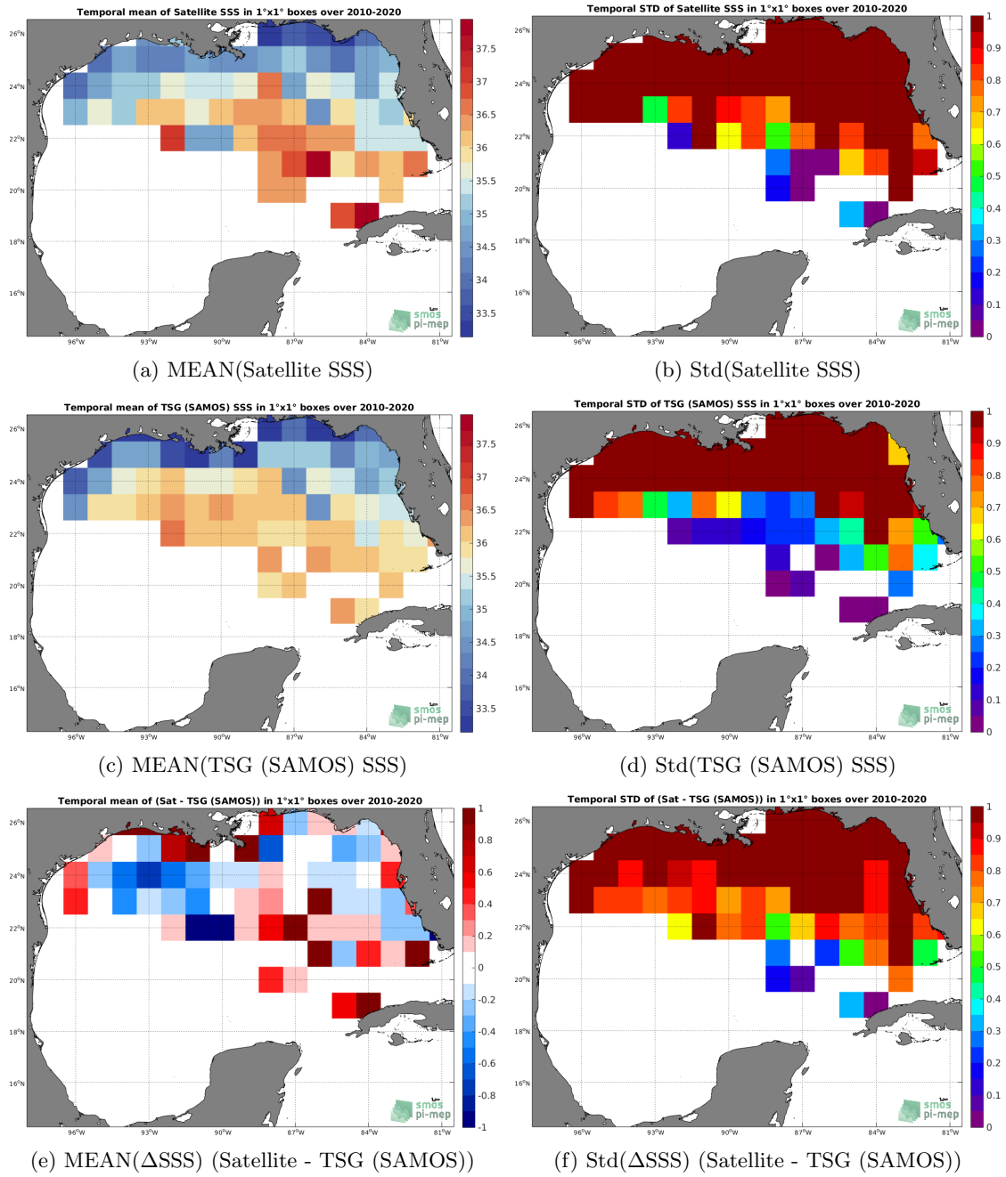
Figure 6: Temporal mean (left) and Std (right) of SSS from SMOS SSS L2Q v330 - 0.25 Deg (CATDS-CPDC) (top), TSG (SAMOS) (middle), and of \Delta SSS (Satellite - TSG (SAMOS)). Only match-up pairs are used to generate these maps.
