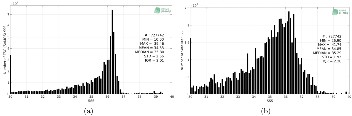
Figure 2: Histograms of SSS from TSG (SAMOS) (a) and SMOS SSS L2Q v330 - 0.25 Deg (CATDS-CPDC) (b) considering all match-up pairs per bins of 0.1 over the Gulf of Mexico Pi-MEP region and for the full satellite product period.
