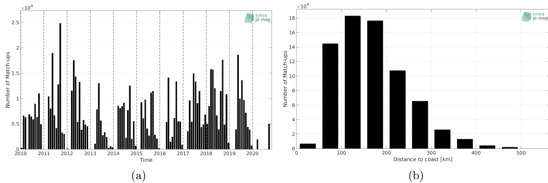
Figure 1: Number of match-ups between TSG (SAMOS) and SMOS SSS L2Q v330 - 0.25 Deg (CATDS-CPDC) SSS as a function of time (a) and as function of the distance to coast (b) over the Gulf of Mexico Pi-MEP region and for the full satellite product period.
