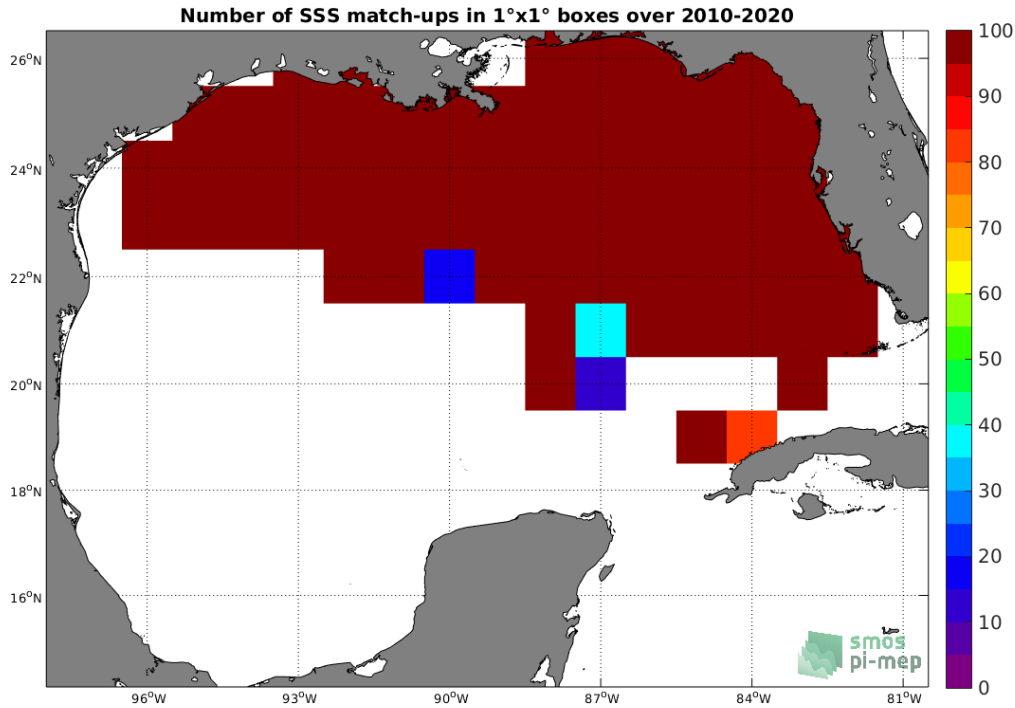
Figure 4: Number of SSS match-ups between TSG (SAMOS) SSS and the SMOS SSS L2Q v330 - 0.25 Deg (CATDS-CPDC) SSS product for the Gulf of Mexico Pi-MEP region over 1^\circ \times 1^\circ boxes and for the full satellite product period.
