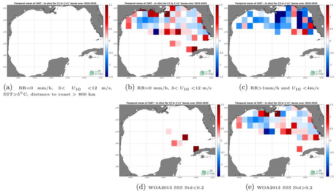
Figure 12: Temporal mean gridded over spatial boxes of size 1^{\circ}\times 1^{\circ} of \Delta\text{SSS} (SMOS SSS L2Q v330 - 0.25 Deg (CATDS-CPDC) - TSG (SAMOS)) for 5 different subdatasets corresponding to:RR=0 mm/h, 3 < U_{10} < 12 m/s, SST >5^{\circ}\text{C} , distance to coast > 800 km (a), RR=0 mm/h, 3 < U_{10} < 12 m/s (b), RR >1 mm/h and U_{10} < 4 m/s (c), WOA2013 SSS Std <0.2 (d), WOA2013 SSS Std >0.2 (e).
