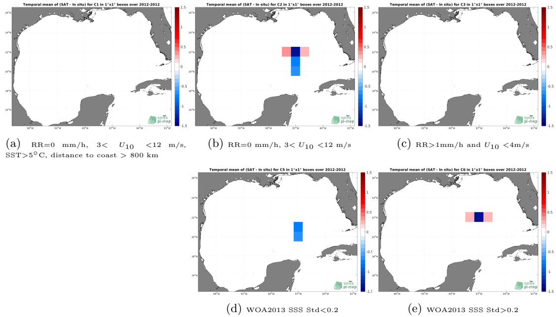
Figure 12: Temporal mean gridded over spatial boxes of size 1^{\circ}\times 1^{\circ} of \Delta SSS (SMOS SSS L2Q v330 - 0.25 Deg (CATDS-CPDC) - TSG (GOSUD-Sailing-ship)) for 5 different subdatasets corresponding to:RR=0 mm/h, 3 < U_{10} < 12 m/s, SST >5^{\circ}\text{C} , distance to coast > 800 km (a), RR=0 mm/h, 3 < U_{10} < 12 m/s (b), RR >1 mm/h and U_{10} < 4 m/s (c), WOA2013 SSS Std <0.2 (d), WOA2013 SSS Std >0.2 (e).
