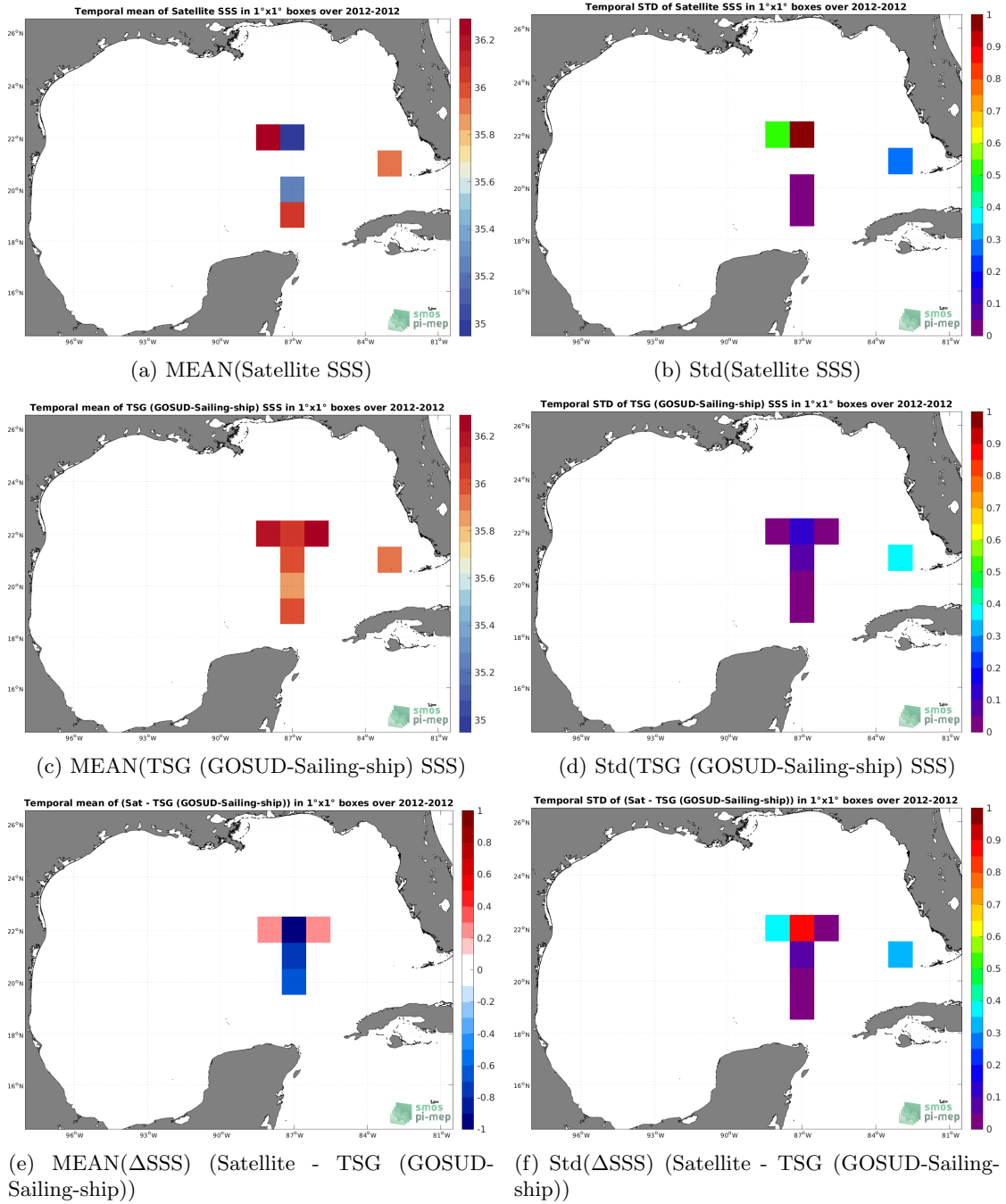
Figure 6: Temporal mean (left) and Std (right) of SSS from SMOS SSS L2Q v330 - 0.25 Deg (CATDS-CPDC) (top), TSG (GOSUD-Sailing-ship) (middle), and of \Delta SSS (Satellite - TSG (GOSUD-Sailing-ship)). Only match-up pairs are used to generate these maps.
