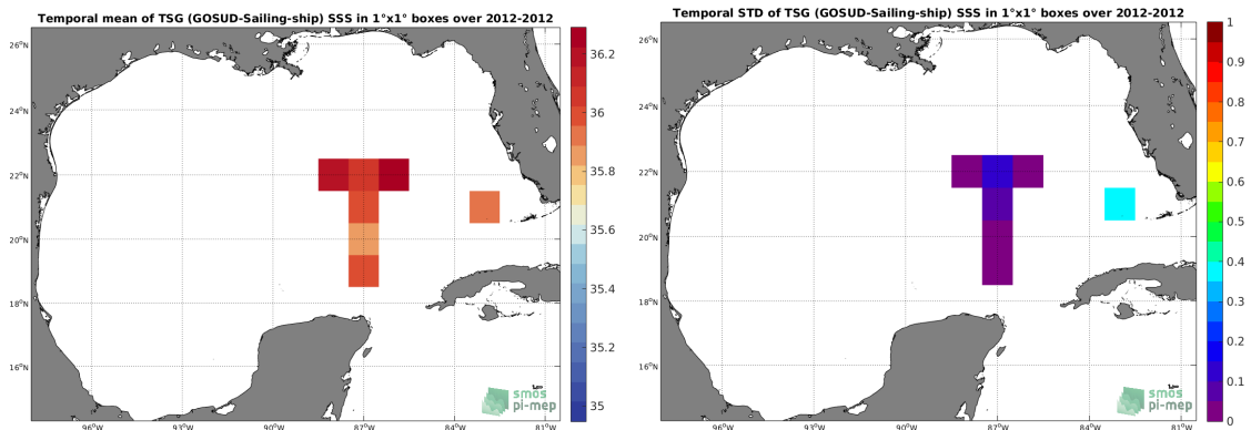
(c) MEAN(TSG (GOSUD-Sailing-ship) SSS)
