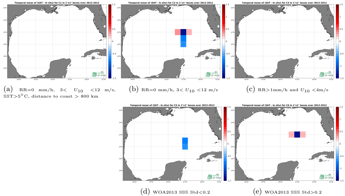
Figure 12: Temporal mean gridded over spatial boxes of size 1^\circ \times 1^\circ of \Delta SSS (SMOS SSS L2Q v330 - 0.25 Deg (CATDS-CPDC) - TSG (GOSUD-Sailing-ship)) for 5 different subdatasets corresponding to:RR=0 mm/h, 3 < U_{10} < 12 m/s, SST >5^\circ\text{C} , distance to coast > 800 km (a), RR=0 mm/h, 3 < U_{10} < 12 m/s (b), RR >1 mm/h and U_{10} < 4 m/s (c), WOA2013 SSS Std <0.2 (d), WOA2013 SSS Std >0.2 (e).
