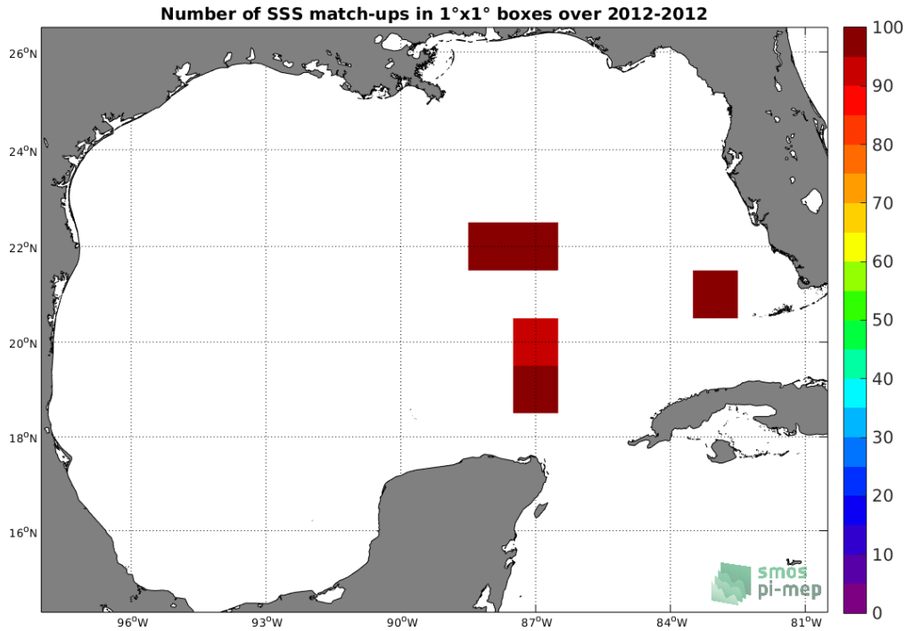
Figure 4: Number of SSS match-ups between TSG (GOSUD-Sailing-ship) SSS and the SMOS SSS L2Q v330 - 0.25 Deg (CATDS-CPDC) SSS product for the Gulf of Mexico Pi-MEP region over 1^\circ \times 1^\circ boxes and for the full satellite product period.
