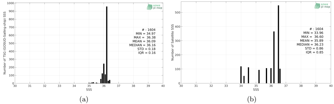
Figure 2: Histograms of SSS from TSG (GOSUD-Sailing-ship) (a) and SMOS SSS L2Q v330 - 0.25 Deg (CATDS-CPDC) (b) considering all match-up pairs per bins of 0.1 over the Gulf of Mexico Pi-MEP region and for the full satellite product period.
