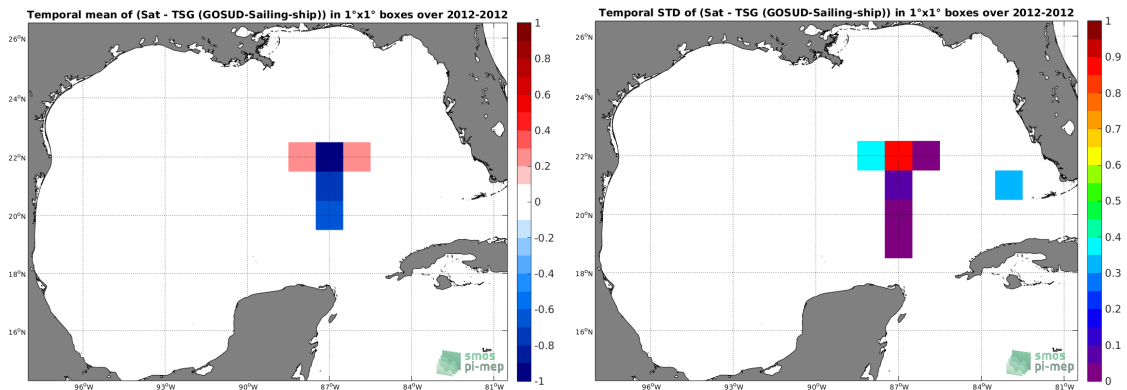
(e) MEAN( \Delta SSS) (Satellite - TSG (GOSUD-Sailing-ship))
