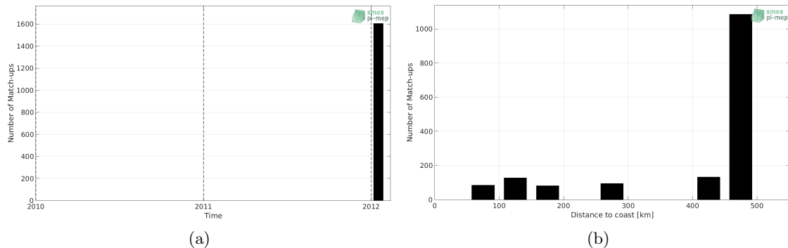
Figure 1: Number of match-ups between TSG (GOSUD-Sailing-ship) and SMOS SSS L2Q v330 - 0.25 Deg (CATDS-CPDC) SSS as a function of time (a) and as function of the distance to coast (b) over the Gulf of Mexico Pi-MEP region and for the full satellite product period.
