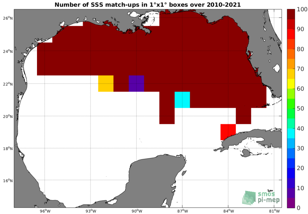
Figure 4: Number of SSS match-ups between TSG (SAMOS) SSS and the SMOS SSS L2Q v321 - 0.25 Deg (CATDS-CPDC) SSS product for the Gulf of Mexico Pi-MEP region over 1^\circ \times 1^\circ boxes and for the full satellite product period.
