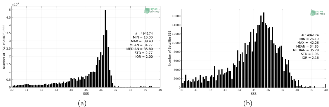
Figure 2: Histograms of SSS from TSG (SAMOS) (a) and SMOS SSS L2Q v321 - 0.25 Deg (CATDS-CPDC) (b) considering all match-up pairs per bins of 0.1 over the Gulf of Mexico Pi-MEP region and for the full satellite product period.
