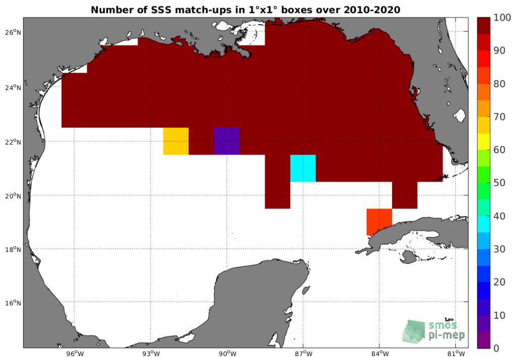
Figure 4: Number of SSS match-ups between TSG (SAMOS) SSS and the SMOS SSS L2Q v321 - 0.25 Deg (CATDS-CPDC) SSS product for the Gulf of Mexico Pi-MEP region over 1°x1° boxes and for the full satellite product period.
