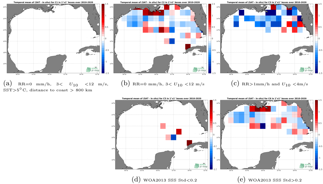
Figure 12: Temporal mean gridded over spatial boxes of size 1^{\circ}\times 1^{\circ} of \Delta\text{SSS} (SMOS SSS L2Q v321 - 0.25 Deg (CATDS-CPDC) - TSG (SAMOS)) for 5 different subdatasets corresponding to:RR=0 mm/h, 3 < U_{10} < 12 m/s, SST >5^{\circ}\text{C} , distance to coast > 800 km (a), RR=0 mm/h, 3 < U_{10} < 12 m/s (b), RR >1 mm/h and U_{10} < 4 m/s (c), WOA2013 SSS Std <0.2 (d), WOA2013 SSS Std >0.2 (e).
