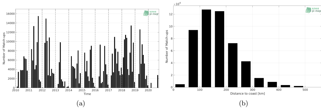
Figure 1: Number of match-ups between TSG (SAMOS) and SMOS SSS L2Q v321 - 0.25 Deg (CATDS-CPDC) SSS as a function of time (a) and as function of the distance to coast (b) over the Gulf of Mexico Pi-MEP region and for the full satellite product period.
