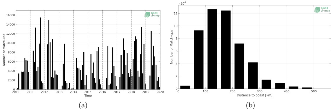
Figure 1: Number of match-ups between TSG-SAMOS and SMOS L2Q v321 - 0.25 Deg (CATDS-CPDC) SSS as a function of time (a) and as function of the distance to coast (b) over the Gulf of Mexico Pi-MEP region and for the full satellite product period.
