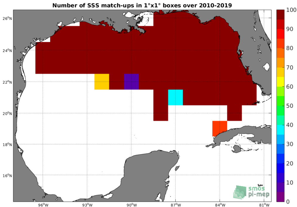
Figure 4: Number of SSS match-ups between TSG-SAMOS SSS and the SMOS L2Q v321 - 0.25 Deg (CATDS-CPDC) SSS product for the Gulf of Mexico Pi-MEP region over 1°x1° boxes and for the full satellite product period.
