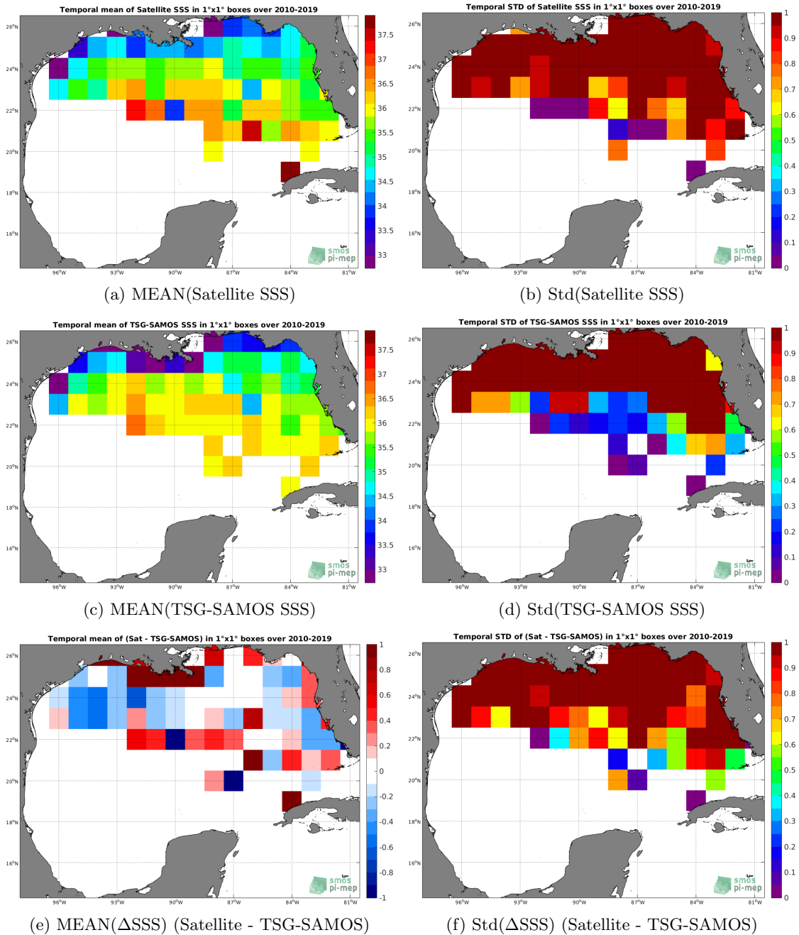
Figure 6: Temporal mean (left) and Std (right) of SSS from SMOS L2Q v321 - 0.25 Deg (CATDS-CPDC) (top), TSG-SAMOS (middle), and of \Delta SSS (Satellite - TSG-SAMOS). Only match-up pairs are used to generate these maps.
