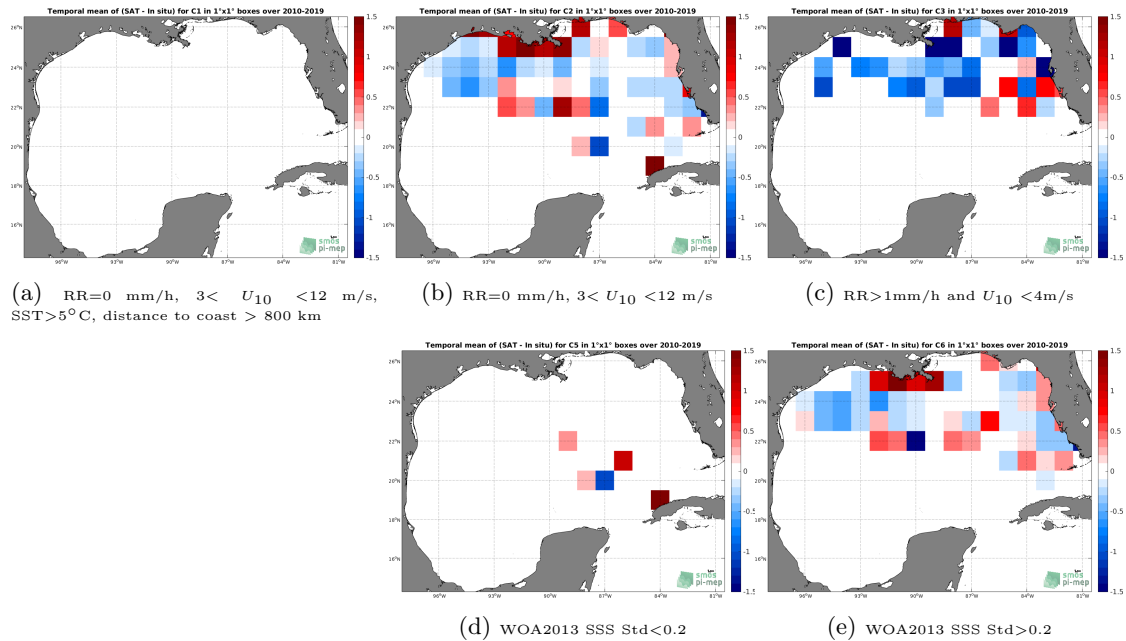
Figure 12: Temporal mean gridded over spatial boxes of size 1^{\circ}\times 1^{\circ} of \Delta\text{SSS} (SMOS L2Q v321 - 0.25 Deg (CATDS-CPDC) - TSG-SAMOS) for 5 different subdatasets corresponding to:RR=0 mm/h, 3 < U_{10} < 12 m/s, SST >5^{\circ}\text{C} , distance to coast > 800 km (a), RR=0 mm/h, 3 < U_{10} < 12 m/s (b), RR >1 mm/h and U_{10} < 4 m/s (c), WOA2013 SSS Std <0.2 (d), WOA2013 SSS Std >0.2 (e).
