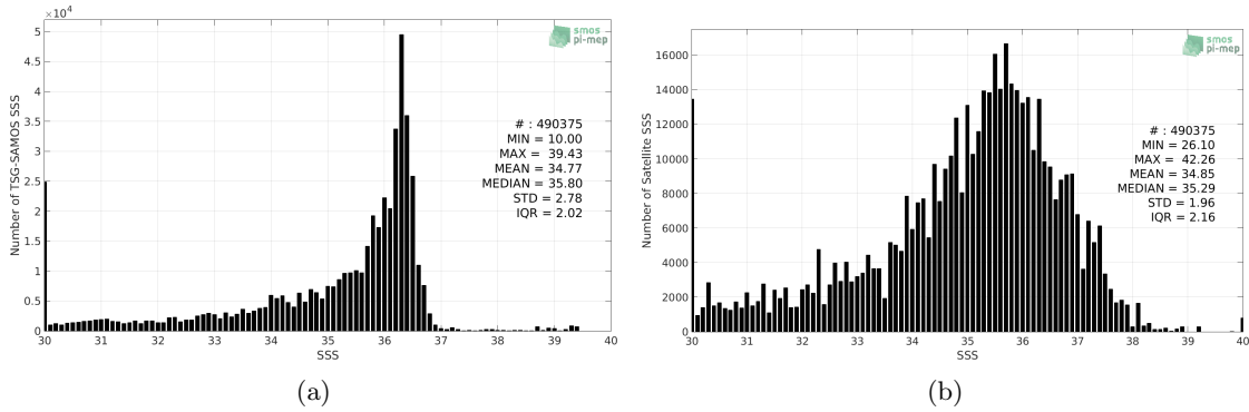
Figure 2: Histograms of SSS from TSG-SAMOS (a) and SMOS L2Q v321 - 0.25 Deg (CATDS-CPDC) (b) considering all match-up pairs per bins of 0.1 over the Gulf of Mexico Pi-MEP region and for the full satellite product period.
