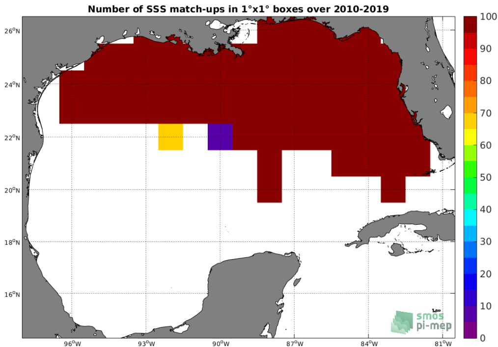
Figure 4: Number of SSS match-ups between TSG-SAMOS SSS and the SMOS-L3-CATDS-CPDC-V321-L2Q SSS product for the Gulf of Mexico Pi-MEP region over 1°x1° boxes and for the full satellite product period.
