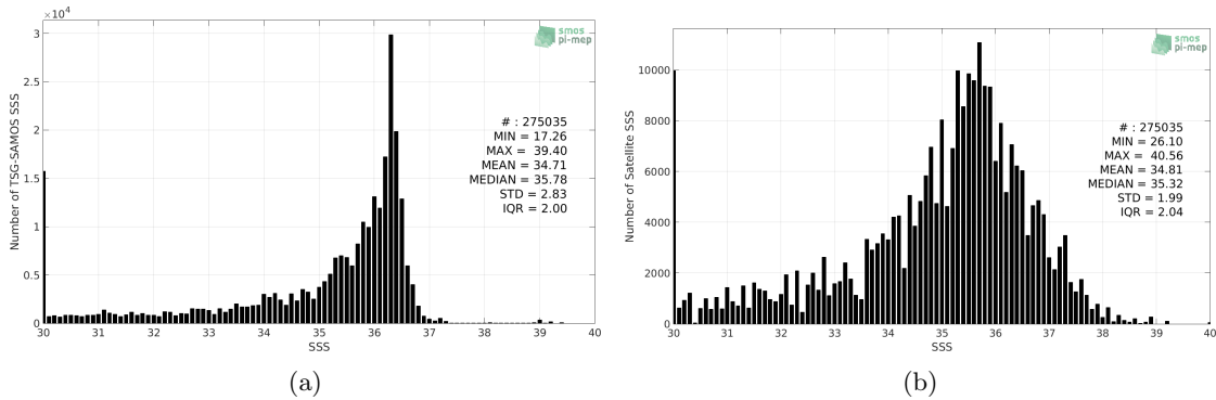
Figure 2: Histograms of SSS from TSG-SAMOS (a) and SMOS-L3-CATDS-CPDC-V321-L2Q (b) considering all match-up pairs per bins of 0.1 over the Gulf of Mexico Pi-MEP region and for the full satellite product period.
