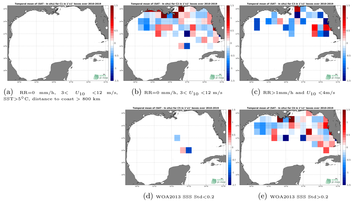
Figure 12: Temporal mean gridded over spatial boxes of size 1^\circ \times 1^\circ of \Delta SSS (SMOS-L3-CATDS-CPDC-V321-L2Q - TSG-SAMOS) for 5 different subdatasets corresponding to:RR=0 mm/h, 3 < U_{10} < 12 m/s, SST >5^\circ C, distance to coast > 800 km (a), RR=0 mm/h, 3 < U_{10} < 12 m/s (b), RR >1 mm/h and U_{10} < 4 m/s (c), WOA2013 SSS Std <0.2 (d), WOA2013 SSS Std >0.2 (e).
