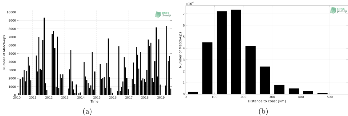
Figure 1: Number of match-ups between TSG-SAMOS and SMOS-L3-CATDS-CPDC-V321-L2Q SSS as a function of time (a) and as function of the distance to coast (b) over the Gulf of Mexico Pi-MEP region and for the full satellite product period.
