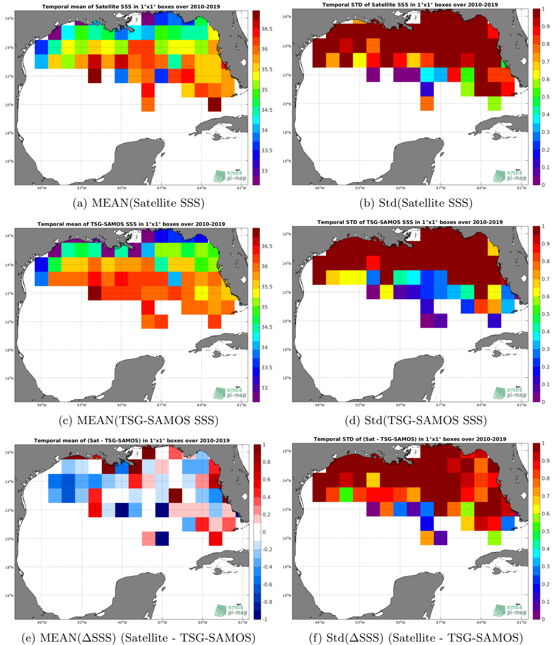
Figure 6: Temporal mean (left) and Std (right) of SSS from SMOS-L3-CATDS-CPDC-V321-L2Q (top), TSG-SAMOS (middle), and of \Delta SSS (Satellite - TSG-SAMOS). Only match-up pairs are used to generate these maps.
