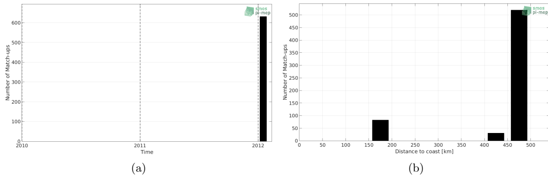
Figure 1: Number of match-ups between TSG (GOSUD-Sailing-ship) and SMOS SSS L2Q v321 - 0.25 Deg (CATDS-CPDC) SSS as a function of time (a) and as function of the distance to coast (b) over the Gulf of Mexico Pi-MEP region and for the full satellite product period.
