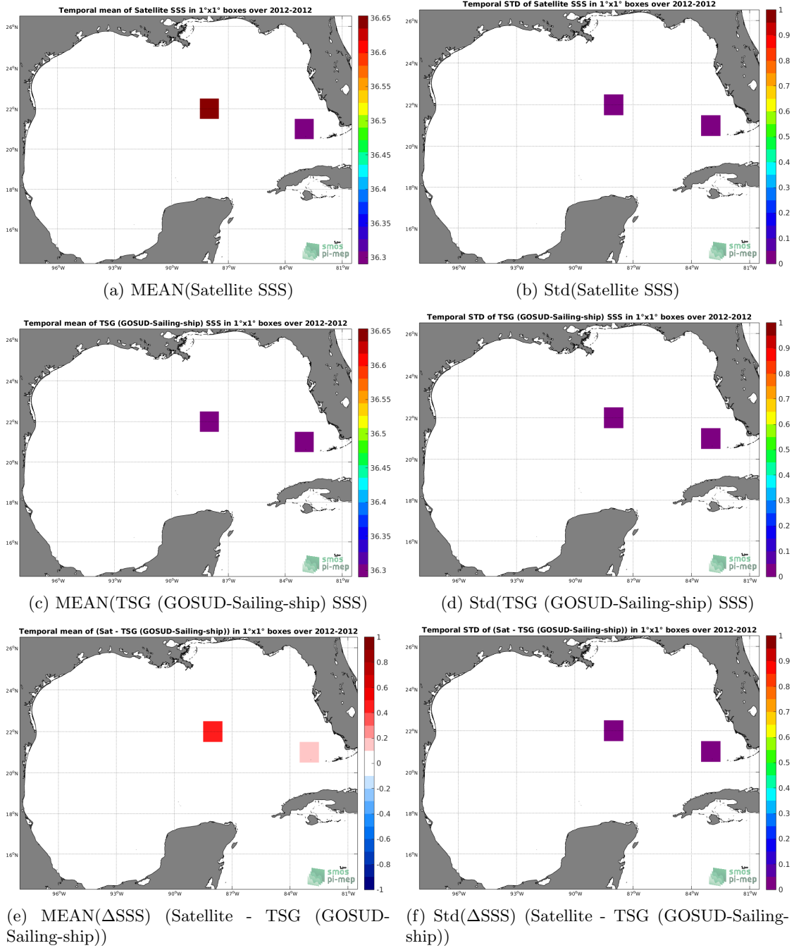
Figure 6: Temporal mean (left) and Std (right) of SSS from SMOS SSS L2Q v321 - 0.25 Deg (CATDS-CPDC) (top), TSG (GOSUD-Sailing-ship) (middle), and of \Delta SSS (Satellite - TSG (GOSUD-Sailing-ship)). Only match-up pairs are used to generate these maps.
