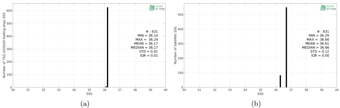
Figure 2: Histograms of SSS from TSG (GOSUD-Sailing-ship) (a) and SMOS SSS L2Q v321 - 0.25 Deg (CATDS-CPDC) (b) considering all match-up pairs per bins of 0.1 over the Gulf of Mexico Pi-MEP region and for the full satellite product period.
