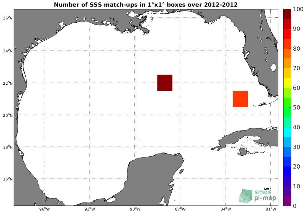
Figure 4: Number of SSS match-ups between TSG (GOSUD-Sailing-ship) SSS and the SMOS SSS L2Q v321 - 0.25 Deg (CATDS-CPDC) SSS product for the Gulf of Mexico Pi-MEP region over 1°x1° boxes and for the full satellite product period.
