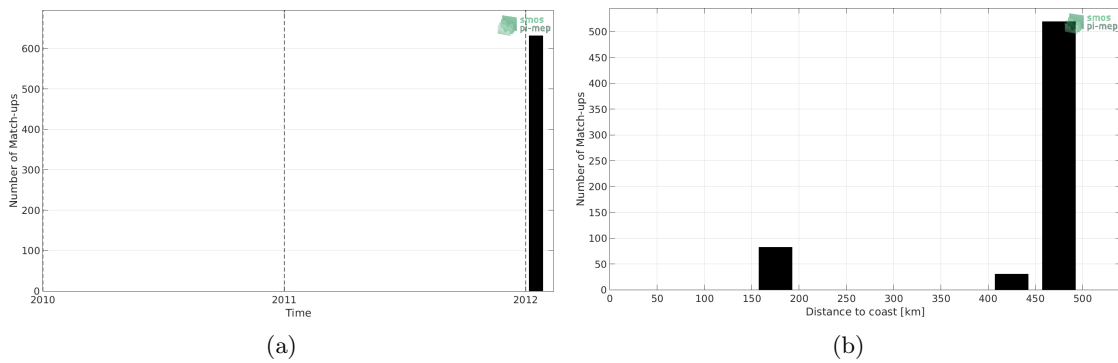
Figure 1: Number of match-ups between TSG (GOSUD-Sailing-ship) and SMOS SSS L2Q v321 - 0.25 Deg (CATDS-CPDC) SSS as a function of time (a) and as function of the distance to coast (b) over the Gulf of Mexico Pi-MEP region and for the full satellite product period.
