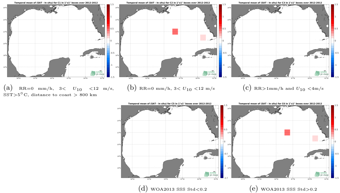
Figure 12: Temporal mean gridded over spatial boxes of size 1^\circ \times 1^\circ of \Delta SSS (SMOS SSS L2Q v321 - 0.25 Deg (CATDS-CPDC) - TSG (GOSUD-Sailing-ship)) for 5 different subdatasets corresponding to:RR=0 mm/h, 3 < U_{10} < 12 m/s, SST >5^\circ\text{C} , distance to coast > 800 km (a), RR=0 mm/h, 3 < U_{10} < 12 m/s (b), RR >1 mm/h and U_{10} < 4 m/s (c), WOA2013 SSS Std <0.2 (d), WOA2013 SSS Std >0.2 (e).
