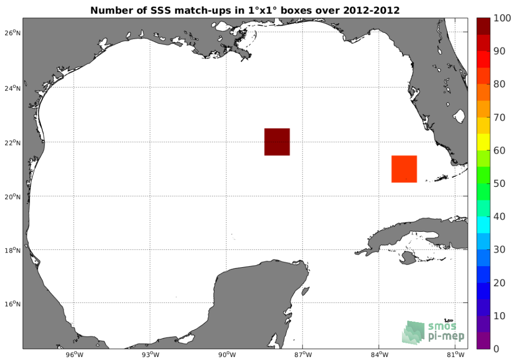
Figure 4: Number of SSS match-ups between TSG-GOSUD-Sailing-ship SSS and the SMOS L2Q v321 - 0.25 Deg (CATDS-CPDC) SSS product for the Gulf of Mexico Pi-MEP region over 1°x1° boxes and for the full satellite product period.
