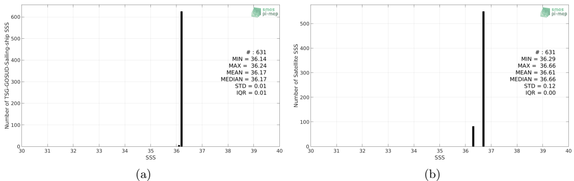
Figure 2: Histograms of SSS from TSG-GOSUD-Sailing-ship (a) and SMOS L2Q v321 - 0.25 Deg (CATDS-CPDC) (b) considering all match-up pairs per bins of 0.1 over the Gulf of Mexico Pi-MEP region and for the full satellite product period.
